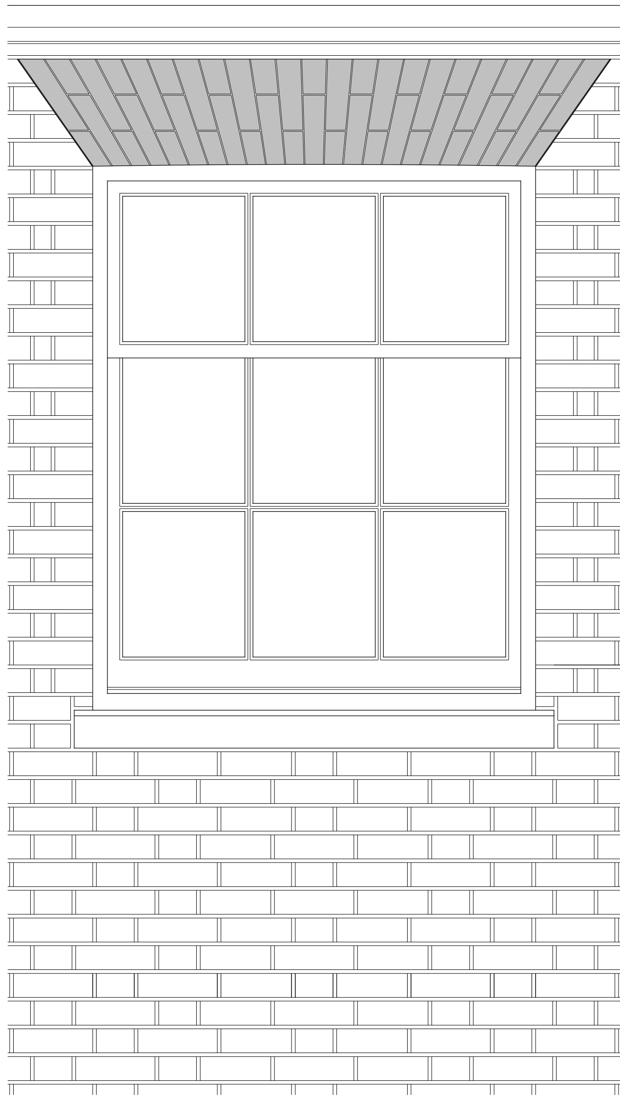
ELEVATION (1:10)
