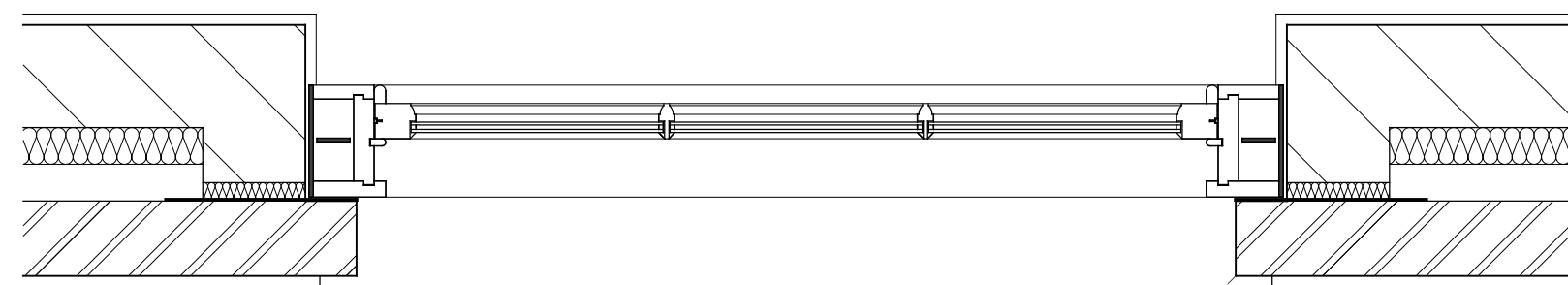
PLAN (1:10)
