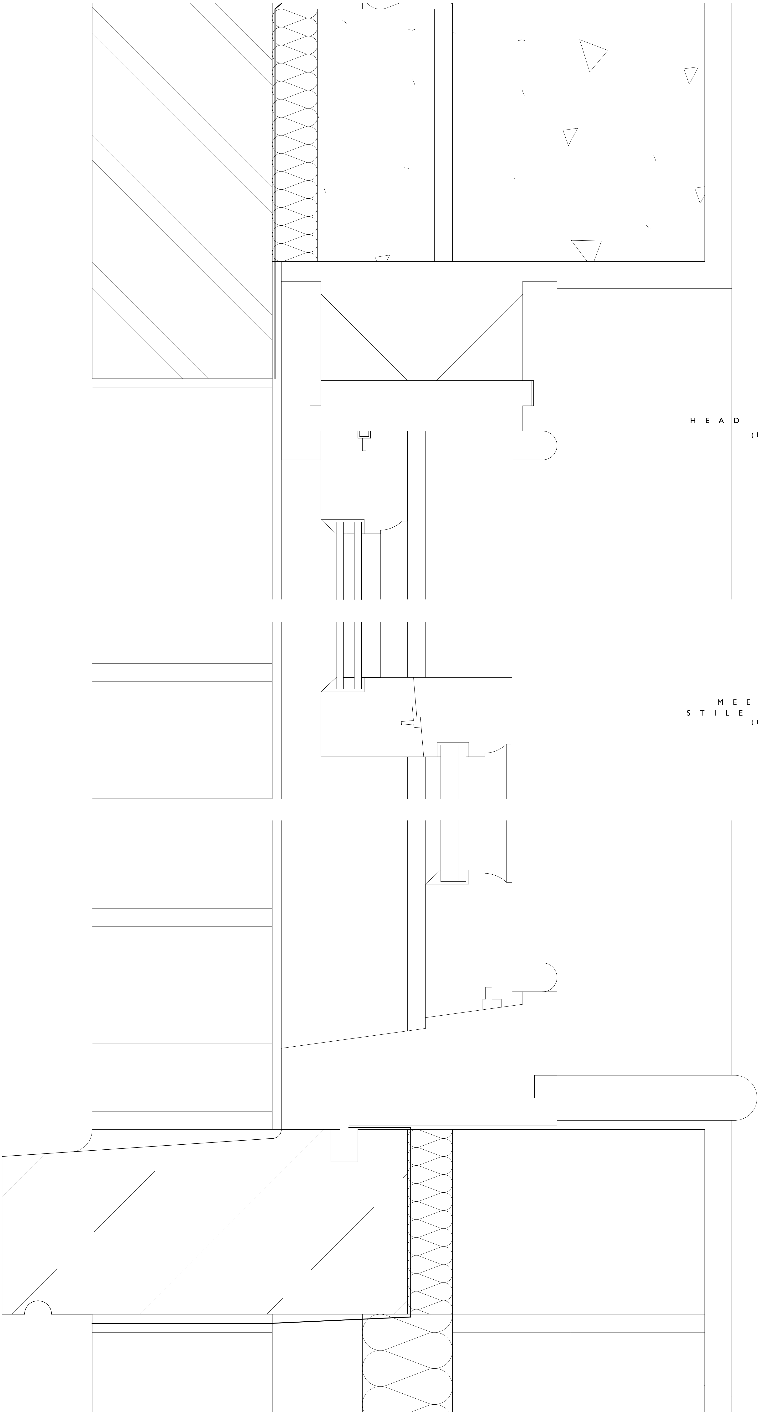
CILL DETAIL (1:1)
