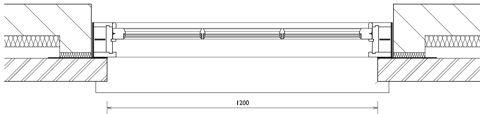
PLAN (1:10)
