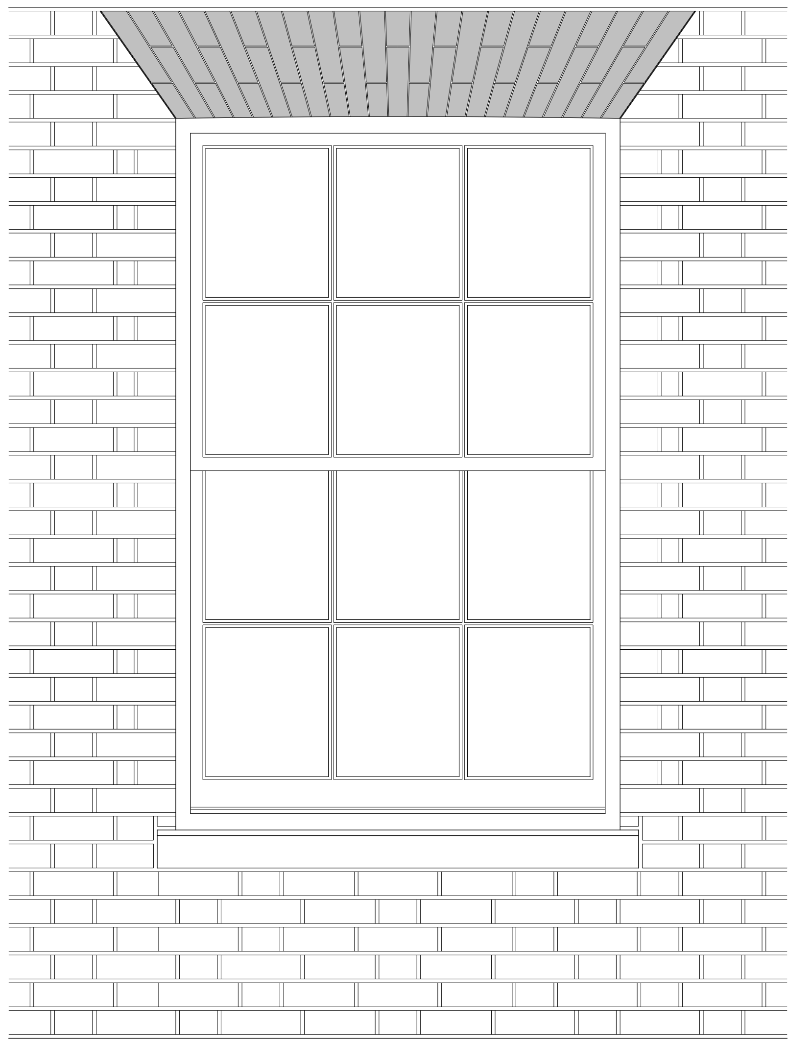
ELEVATION (1:10)
