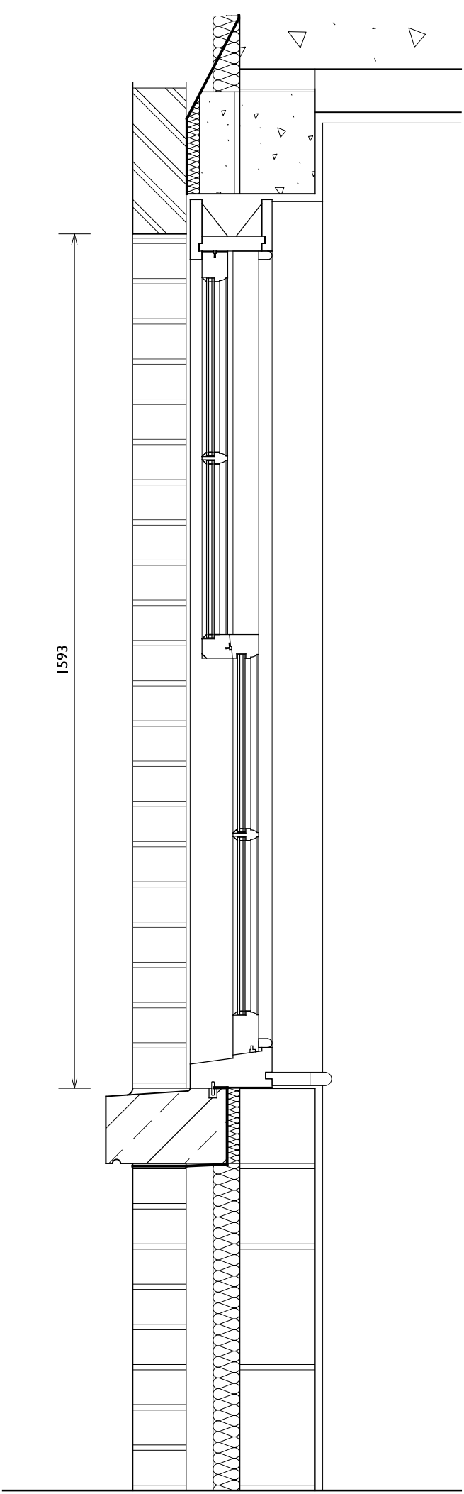
SECTION (1:10)
