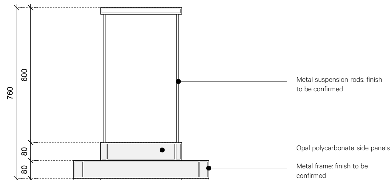
1 Chandelier Side Elevation 1:10 @ A3
