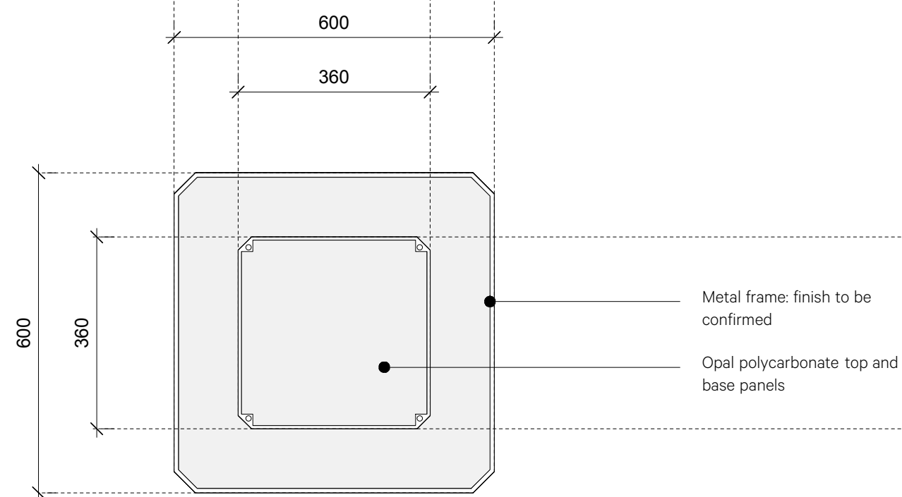
2 Chandelier Top Plan 1:10 @ A3
