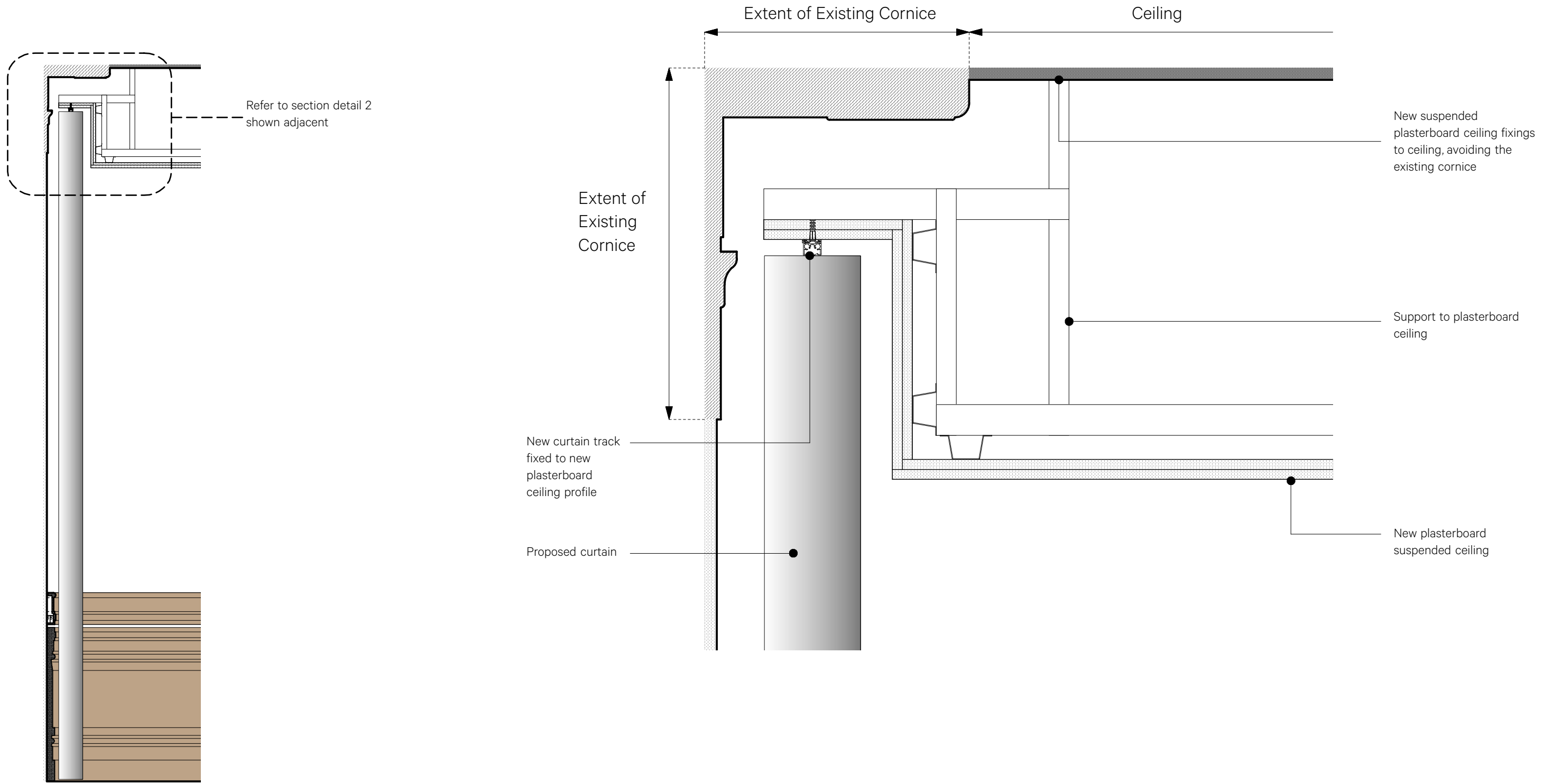
1 Room G.05: Typical section Through Wall / Ceiling 1:20@A3
