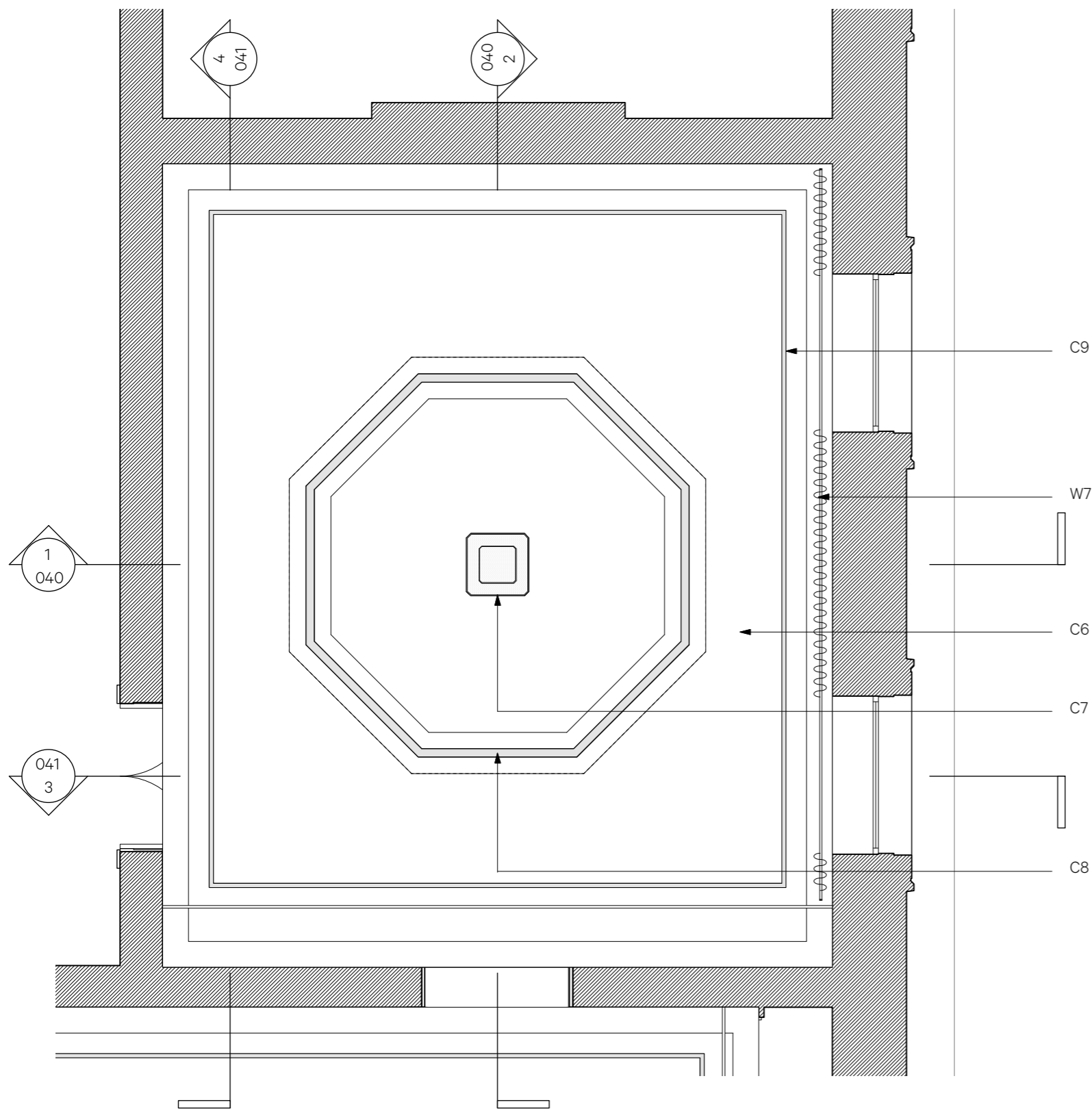
1 G.04: Proposed RCP 1:50@A3
