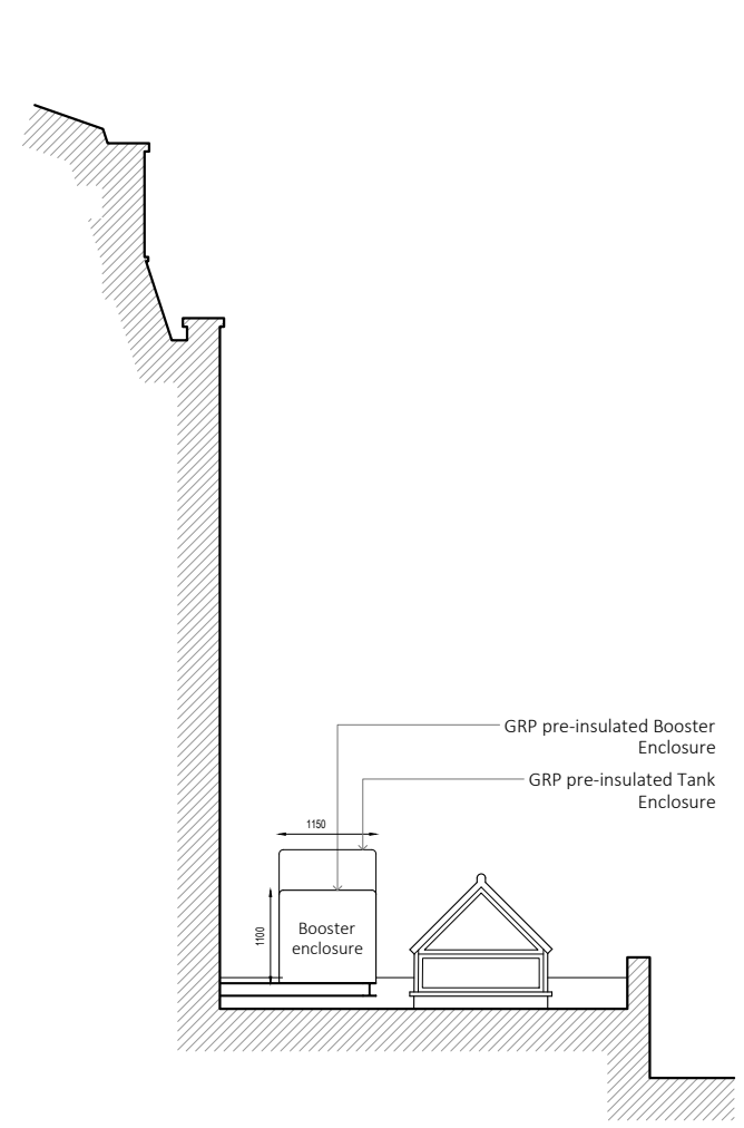
SIDE ELEVATION 02
