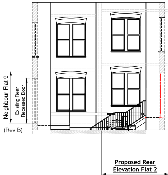
Proposed Elevations
