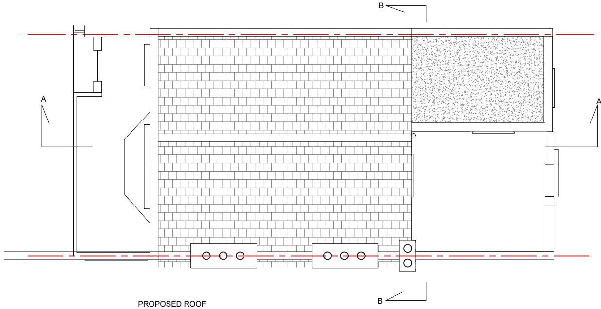
PROPOSED ROOF
