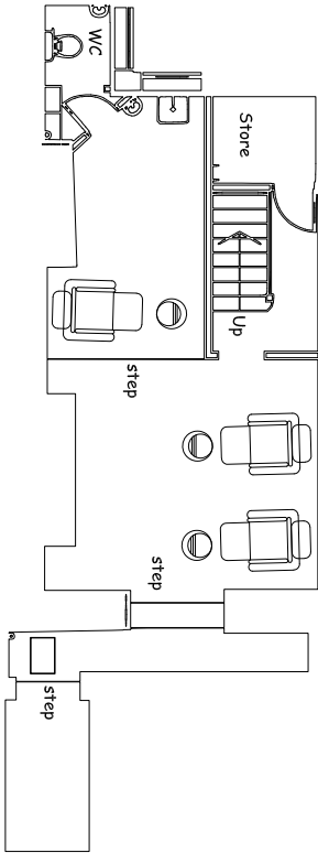
Proposed Basement Floor Plan (1:100)
