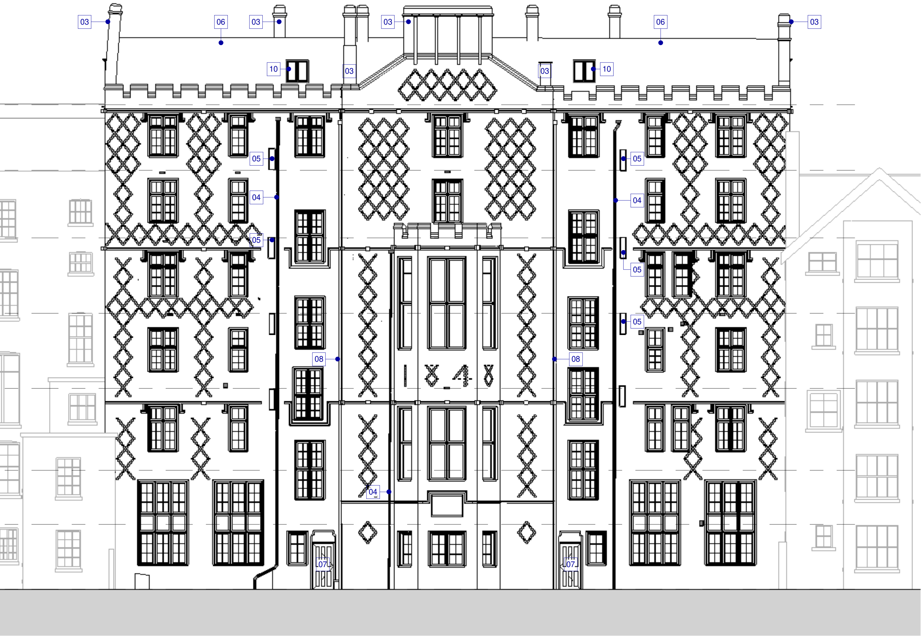
Proposed GA Elevation - Rear
