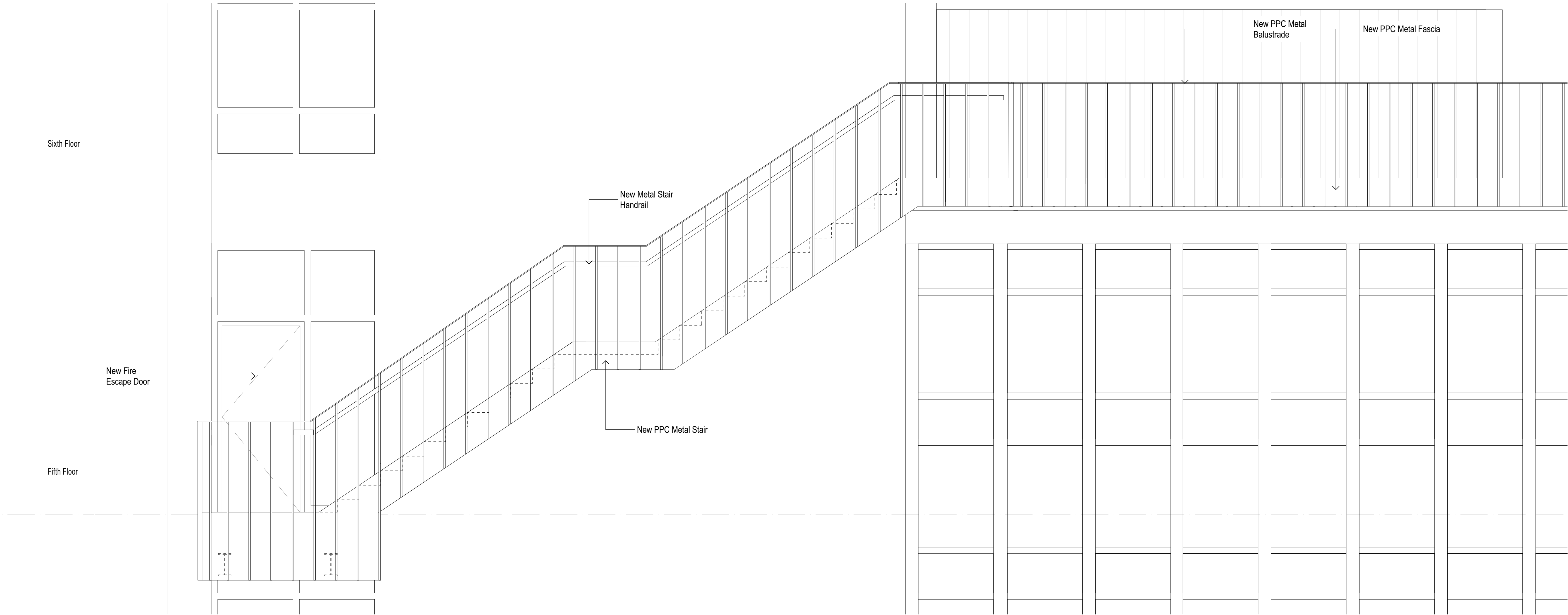
2 Proposed Terrace Detail Elevation, L6 SCALE 1:25
