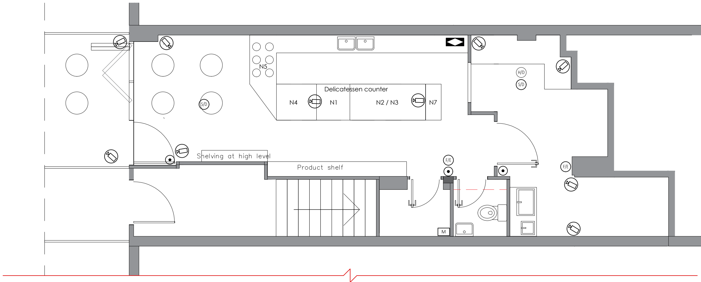
01 Proposed Ground Floor Plan 1:50 @ A3
