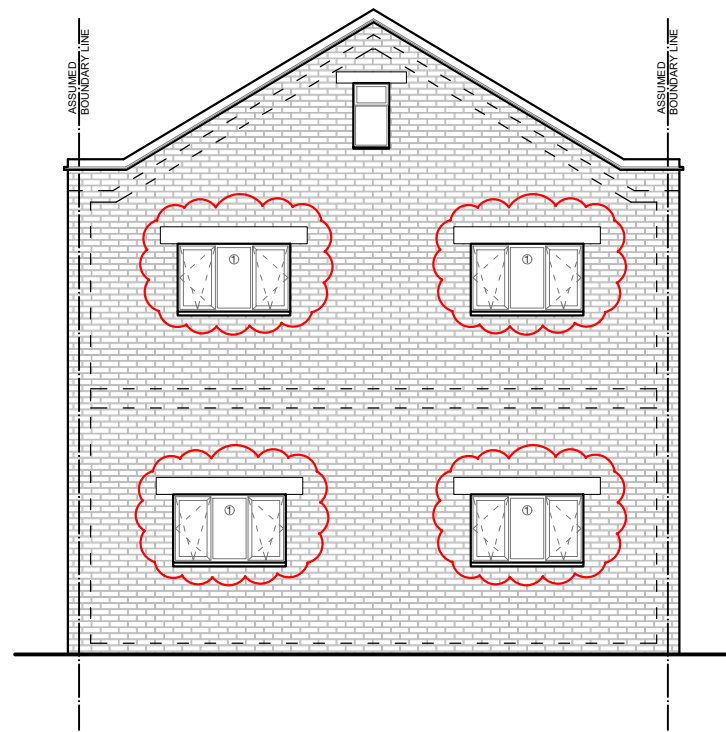
02 PROPOSED REAR ELEVATION A-(10)-010 1:50@ A1,1:100 @ A3
