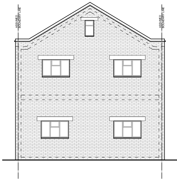
01 EXISTING REAR ELEVATION A-(10)-010 1:50@ A1,1:100 @ A3
