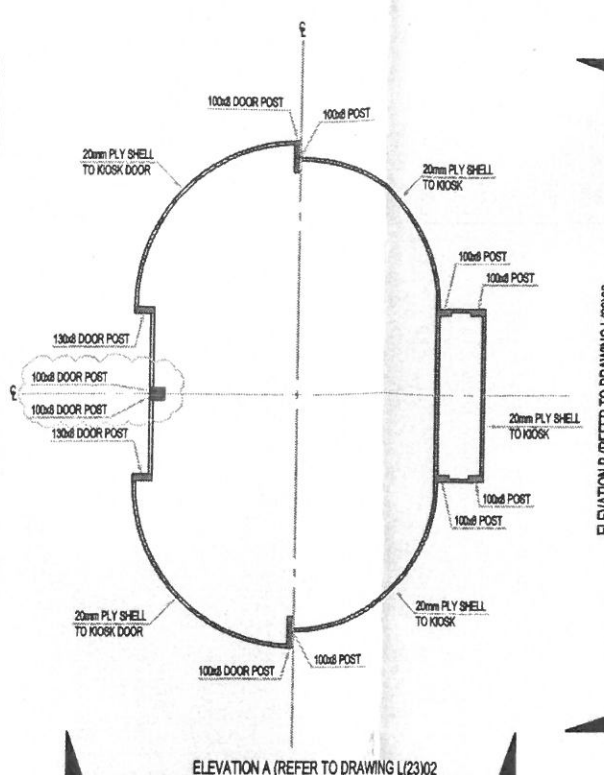
LEVEL 3 PLAN 1:25
