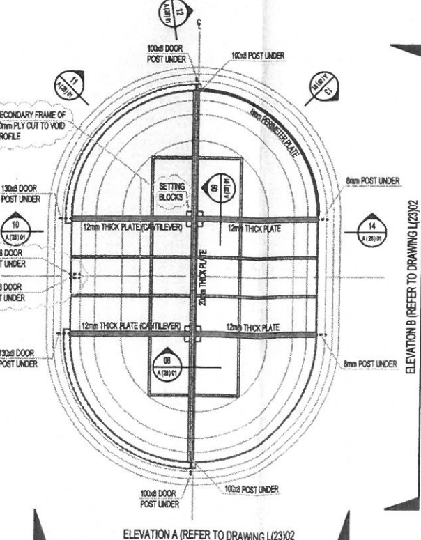
ROOF PLAN 1:25
