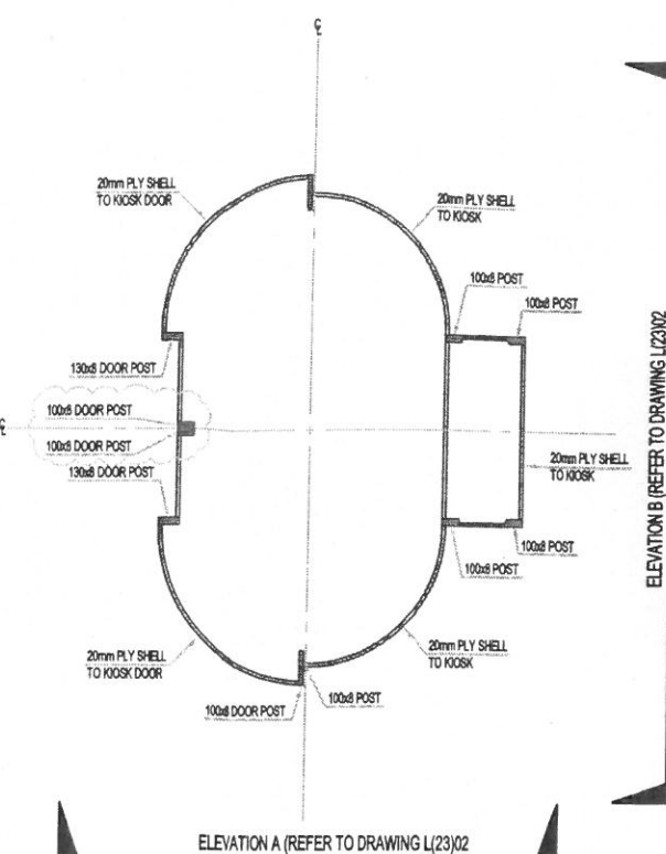
LEVEL 2 PLAN 1:25
