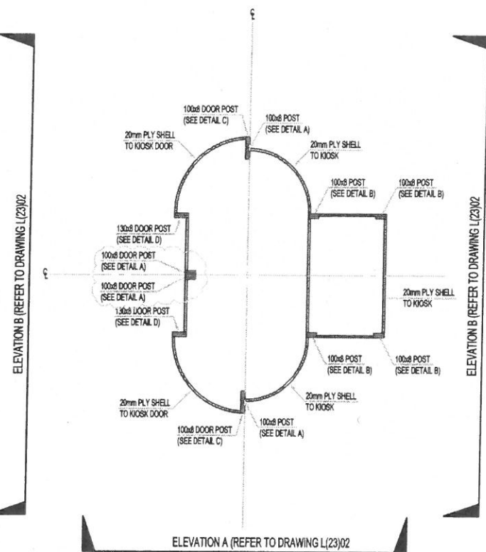
LEVEL 1 PLAN 1:25
