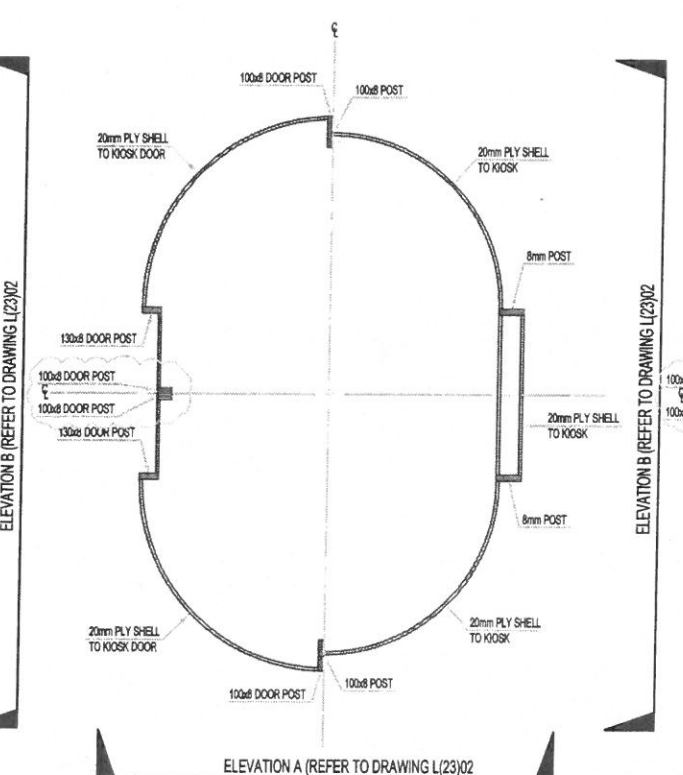
LEVEL 5 PLAN 1:25
