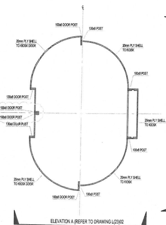
LEVEL 4 PLAN 1:25
