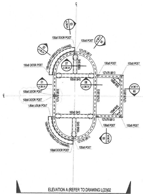
FLOOR STEEL PLAN 1:25
