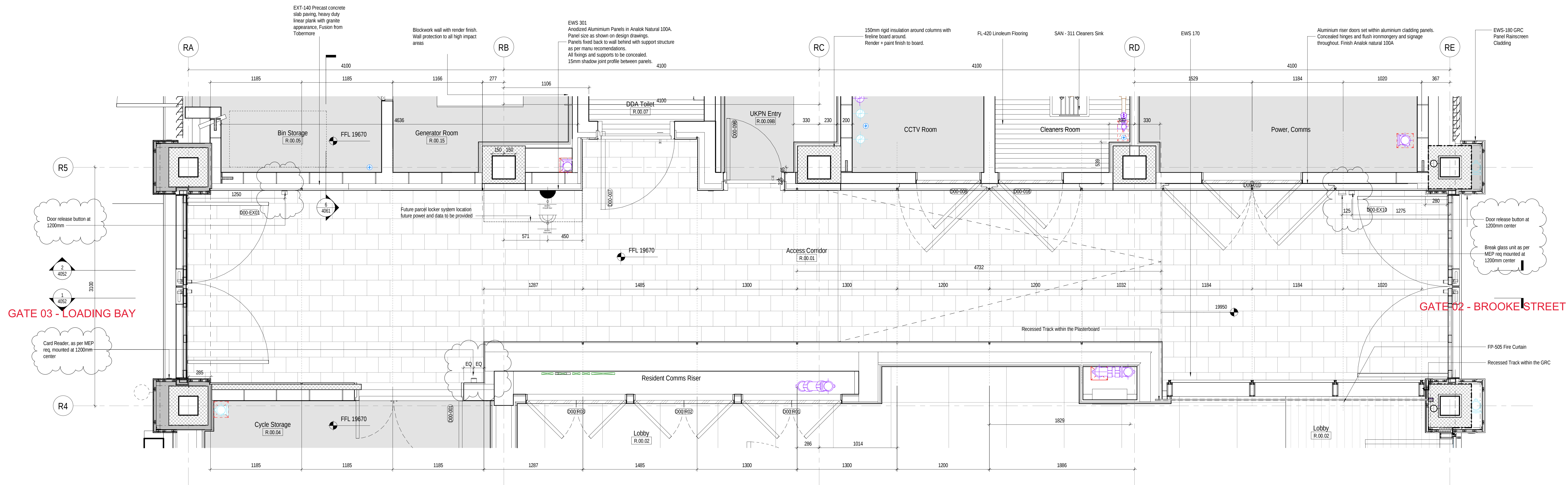
1 Access Corridor Enlarged Plan 1 : 20
