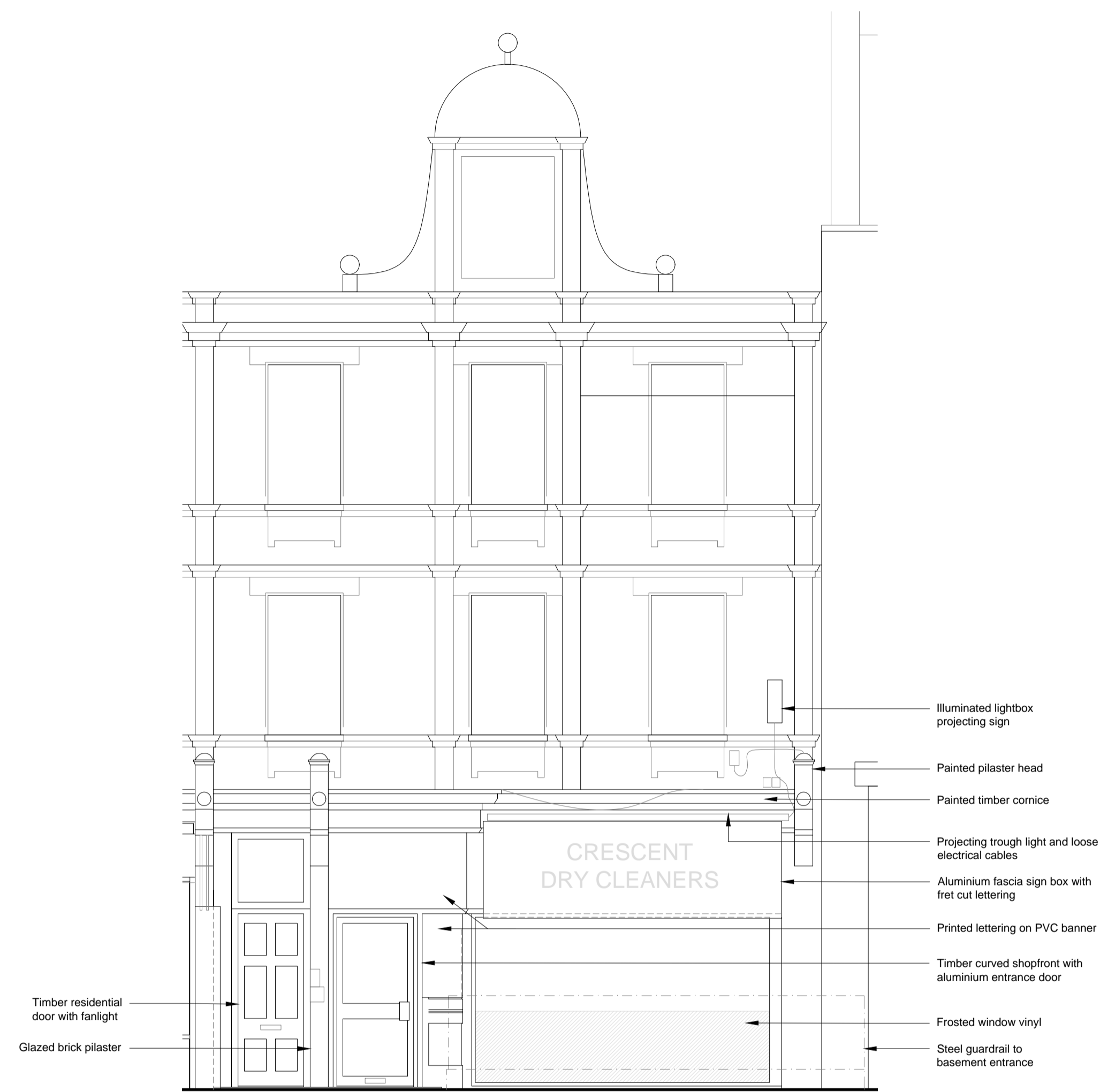
01 Existing Elevation
