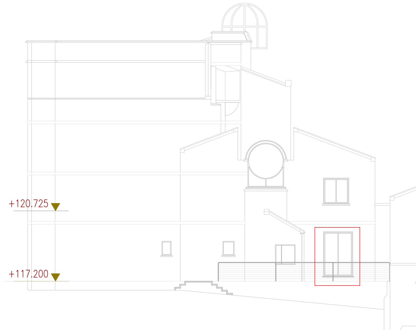
Proposed elevation
