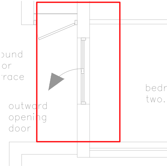
Proposed door detail Scale 1:50@A3
