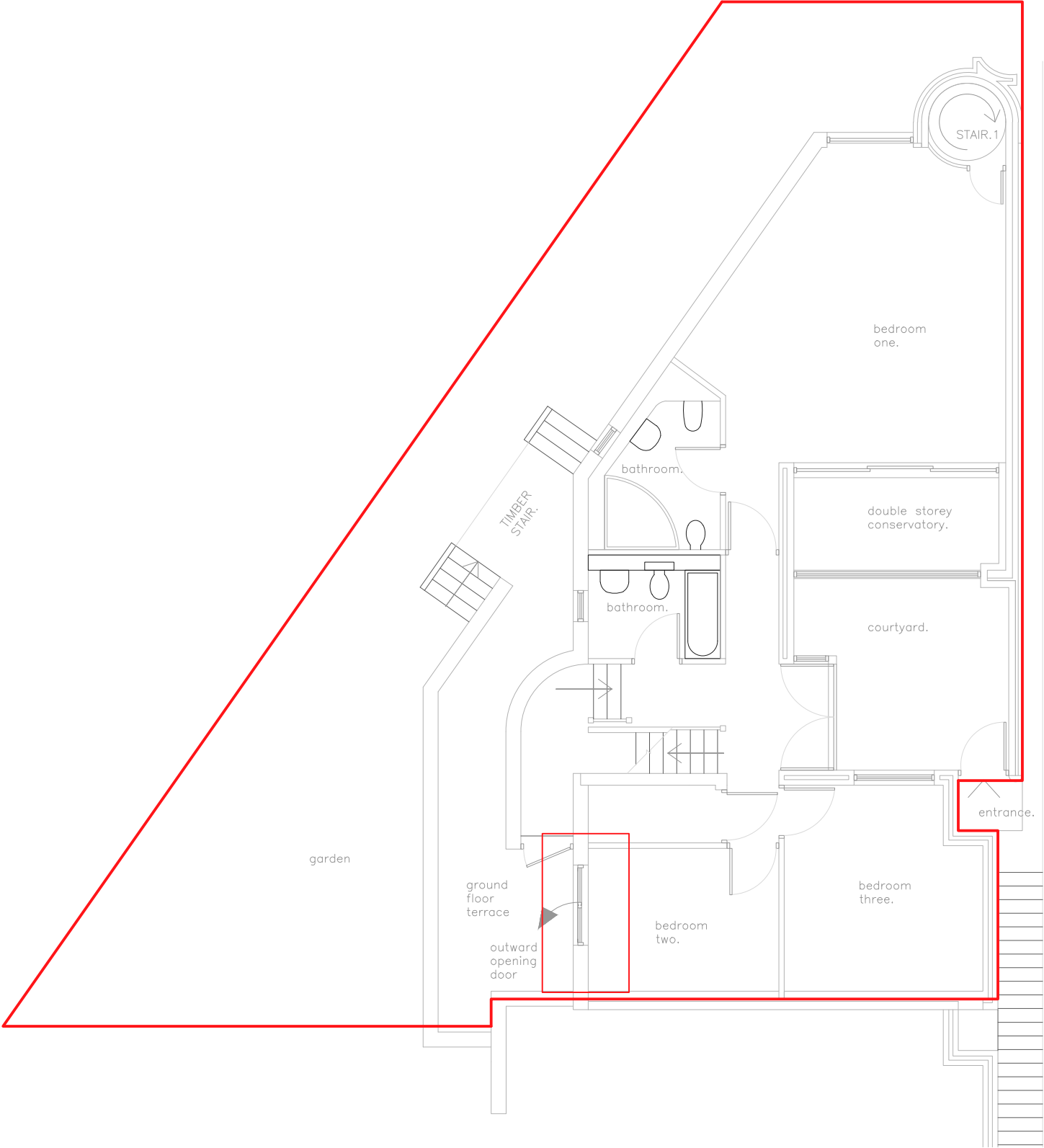
Proposed plan Scale 1:100@A3
