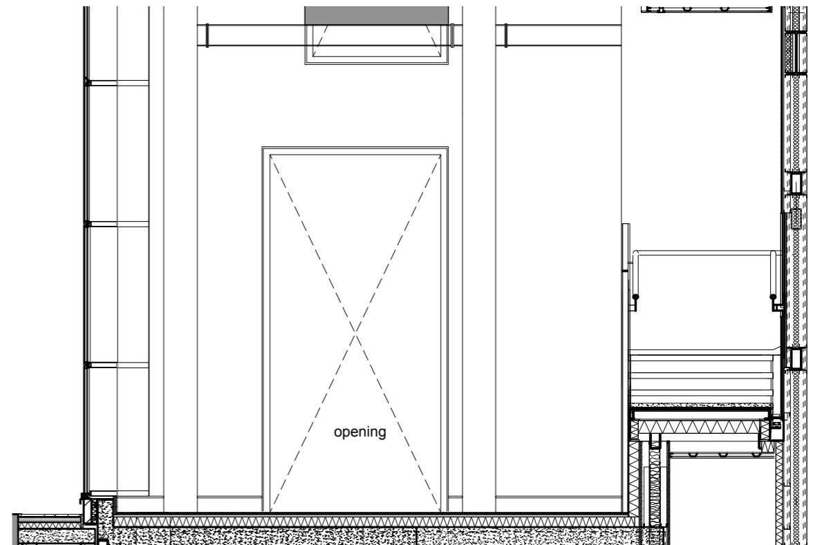
Elevation within Kings Cross Bridge
