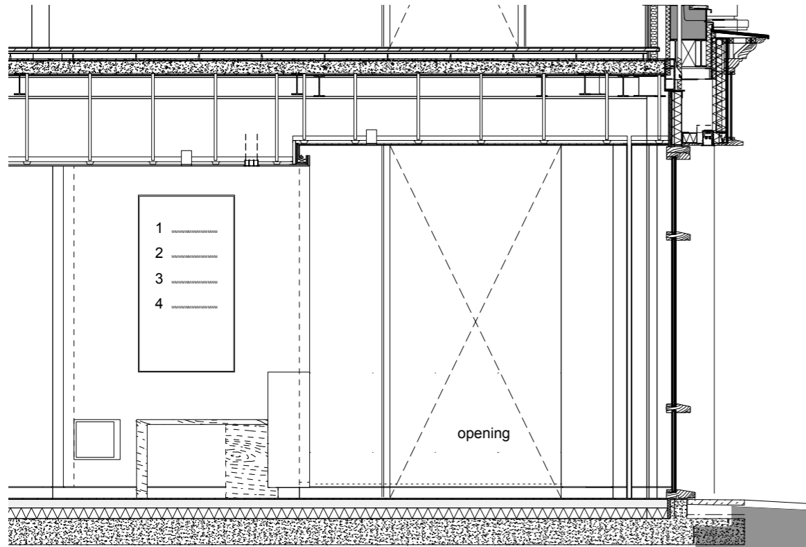
Elevation within the Lighthouse
