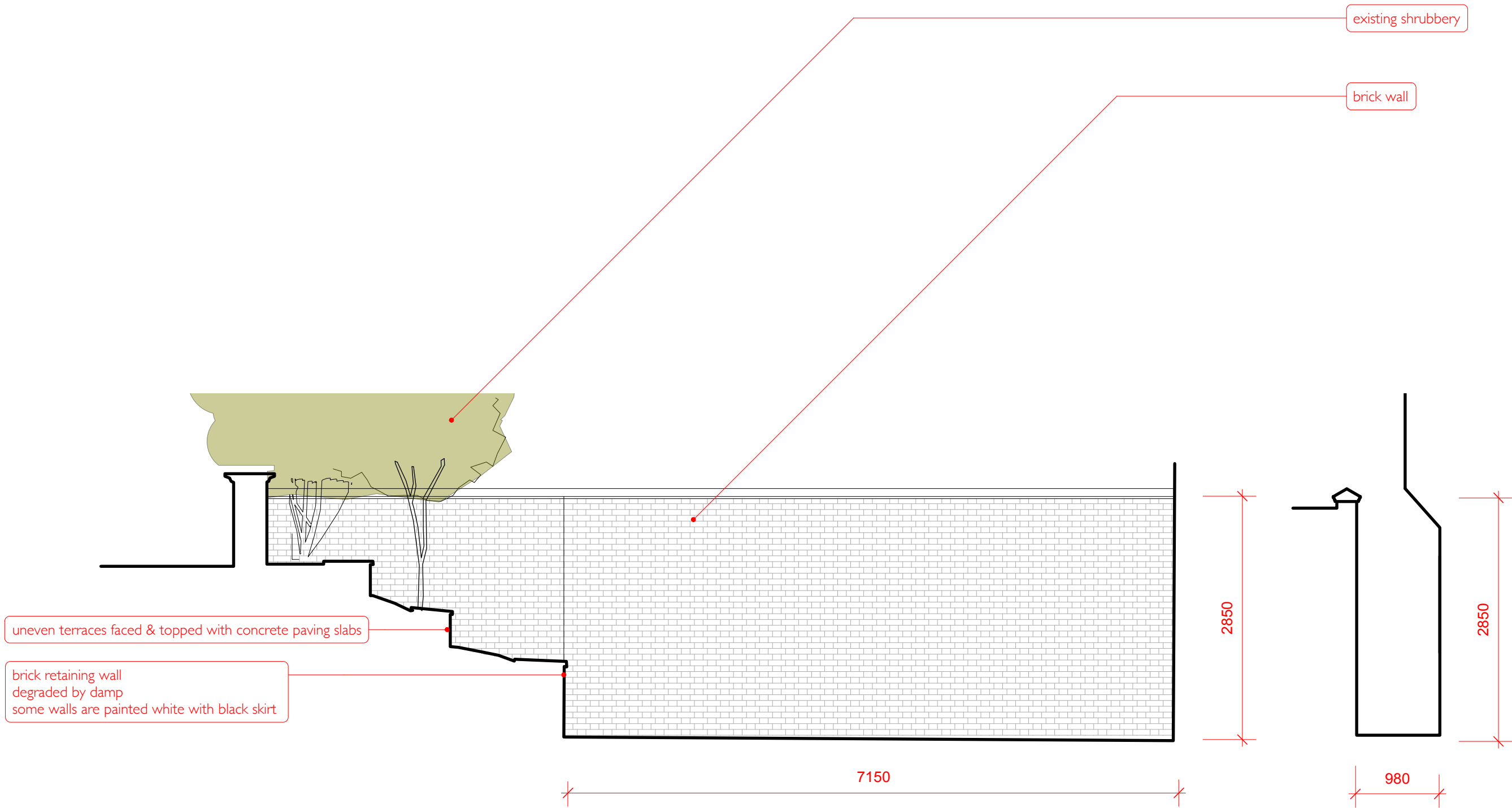
1 Long Elevation (side return) existing 1:50@ A3
