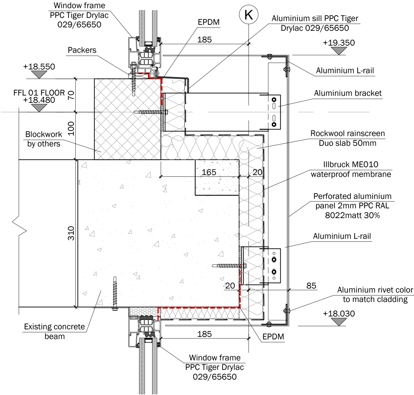
DETAIL 17
