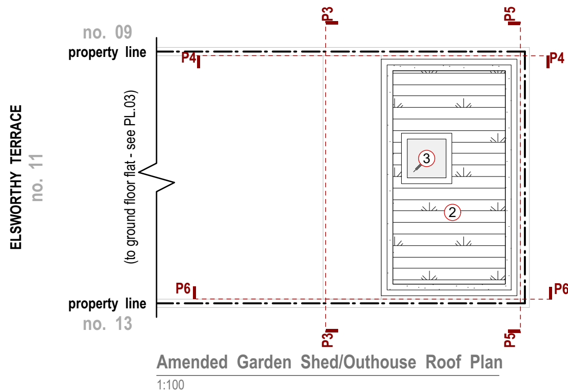
Amended Garden Shed/Outhouse Plan 1:100
