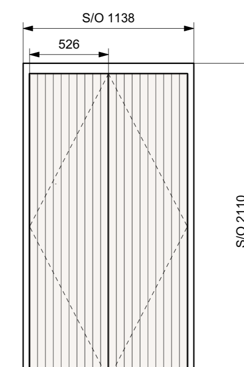
BESPOKE TIMBER BIN STORE DOOR
