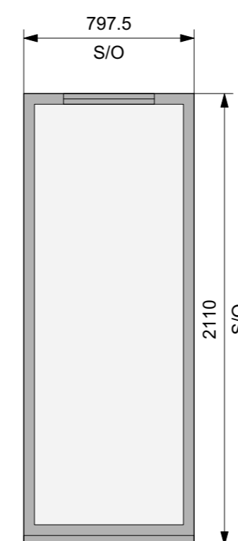
FIXED CASEMENT WINDOW
