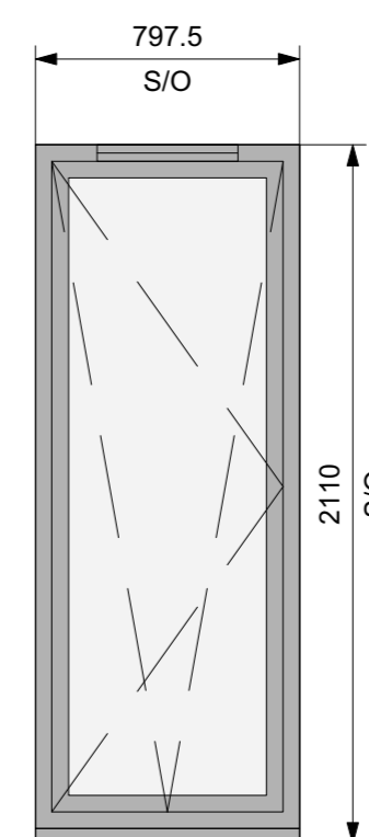
INWARD TILT AND TURN WINDOW
