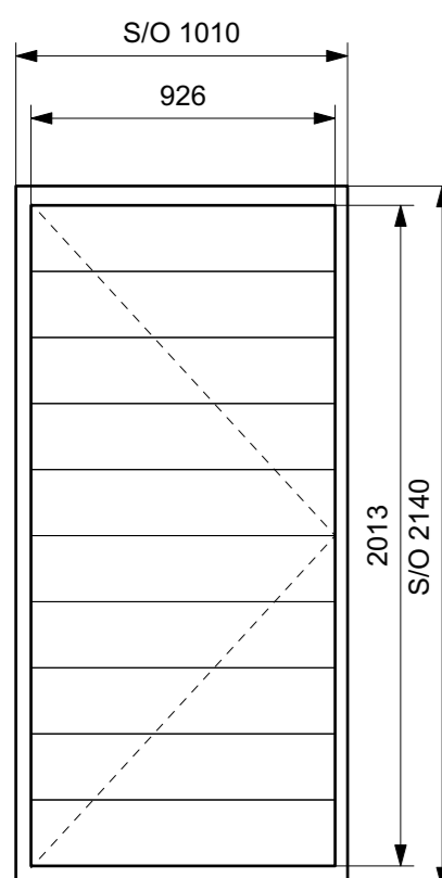
KLOEBER FUNKY FRONT CONTEMPORARY WOODEN ENTRANCE DOOR
