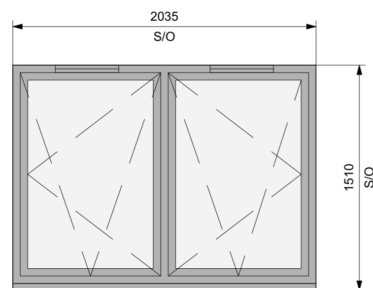
INWARD OPENING TILT AND TURN WINDOW
