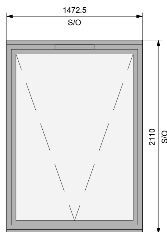
BOTTOM HUNG INWARD TILTING WINDOW
