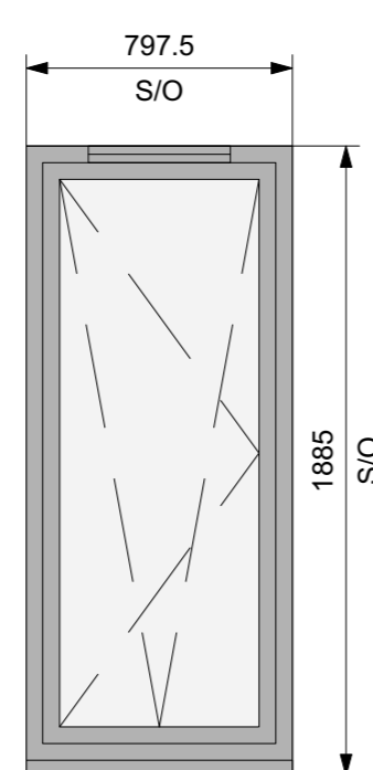
INWARD OPENING TILT AND TURN
