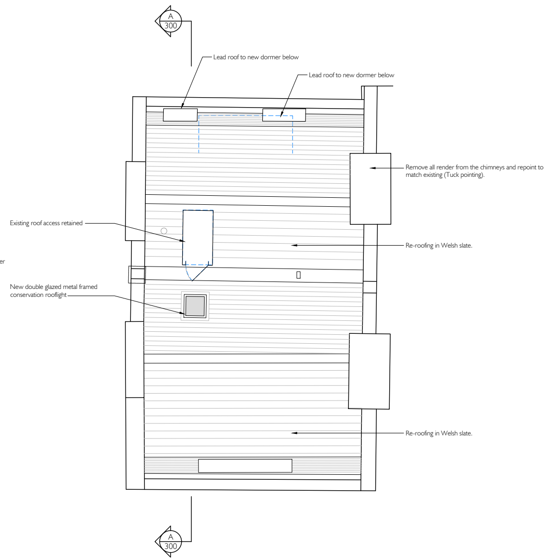
C ROOF PLAN 101 AS PROPOSED
