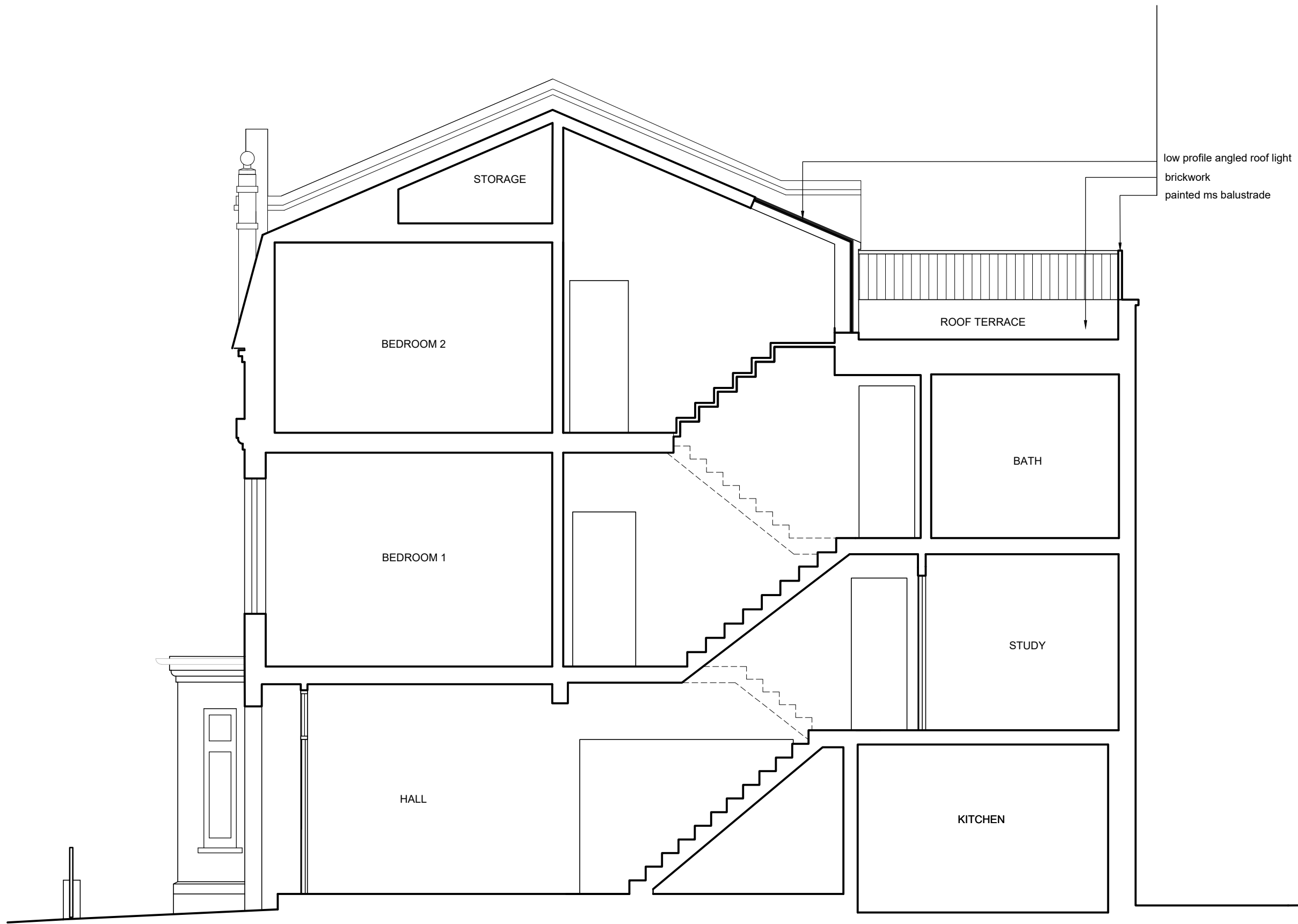
Section C - C
