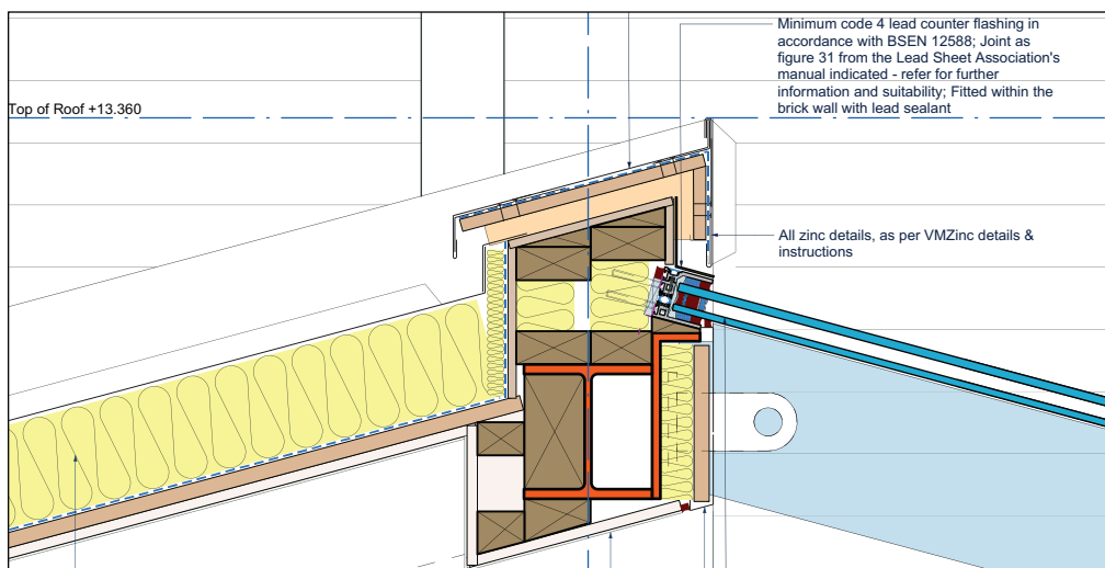
Detail 5 - Rooflight Head, Scale 1:10
