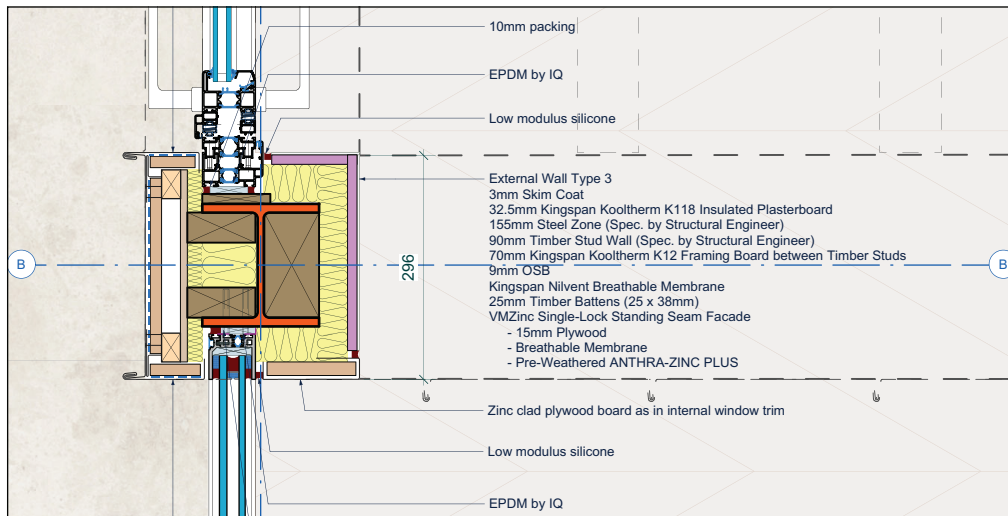
Detail 3 - Fixed Glazing and Bi-Fold Door Jamb, Scale 1:10
