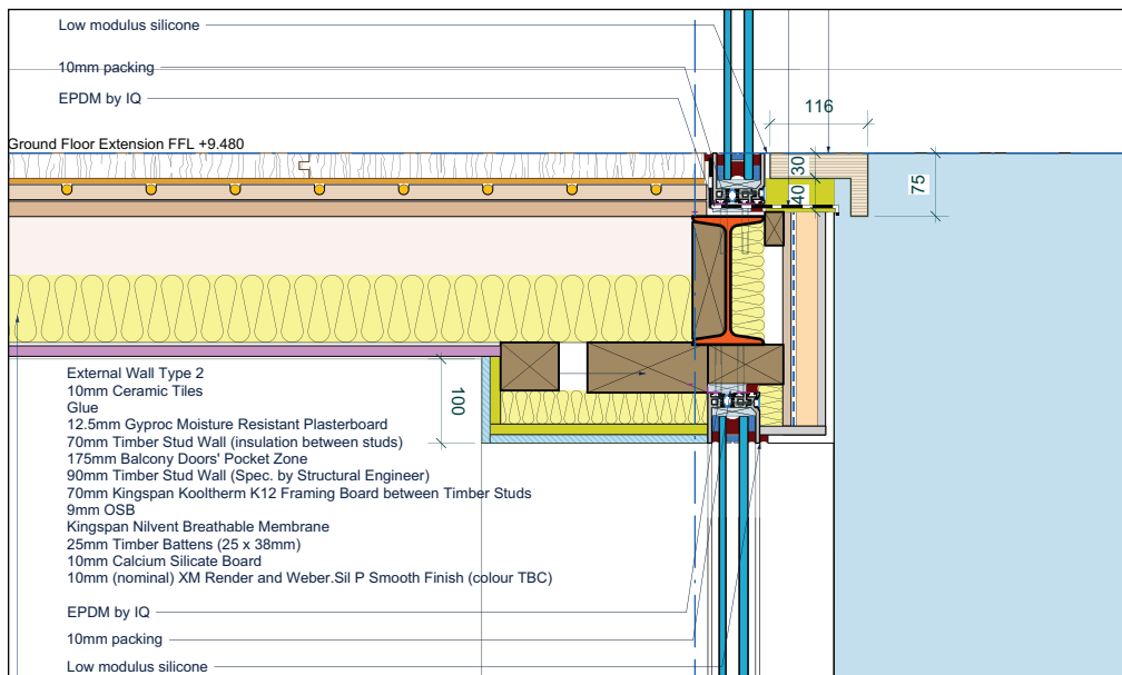
Detail 4 - Fixed Glazing Head & Cill, Scale 1:10
