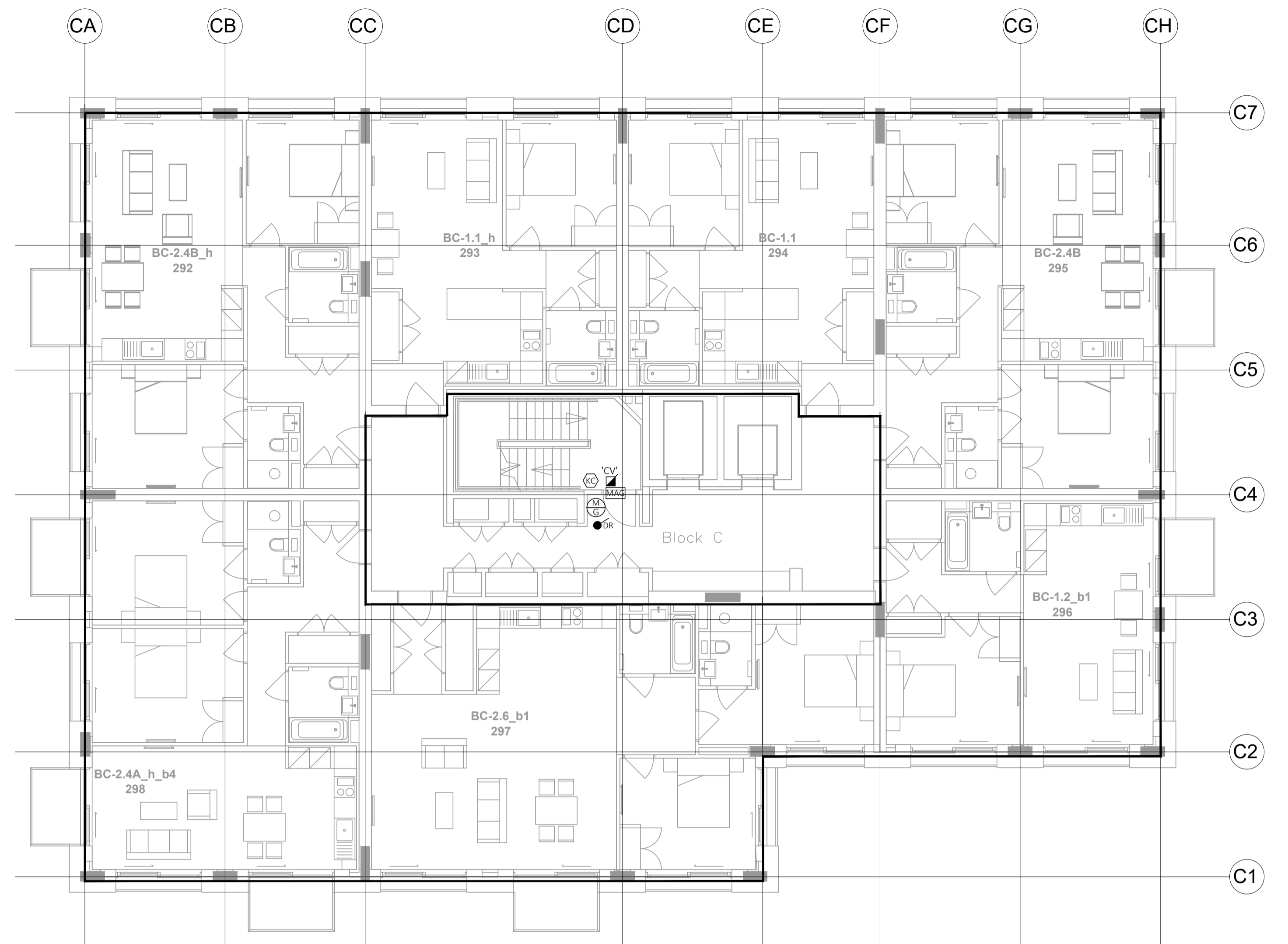
BLOCK C - LEVEL 03
