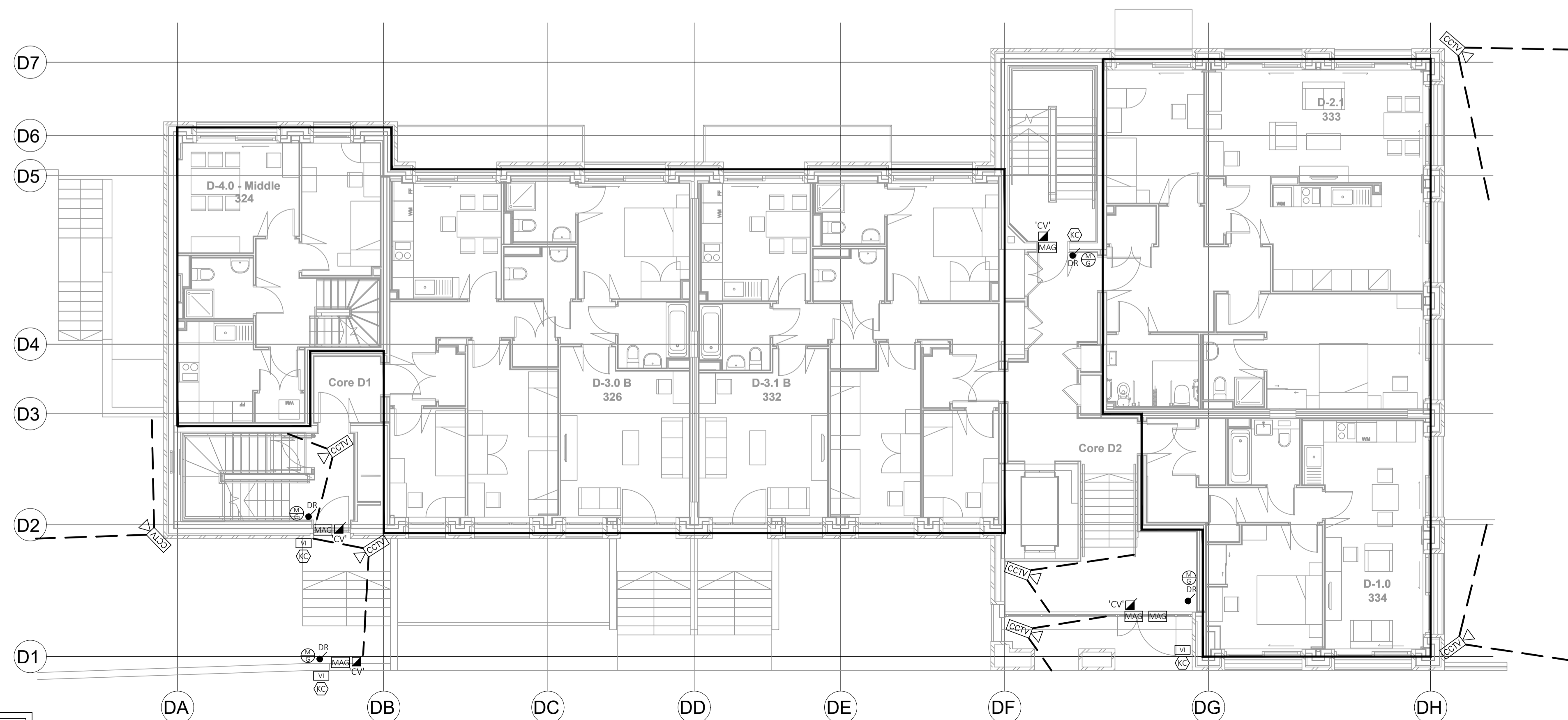
BLOCK D - LEVEL 01
