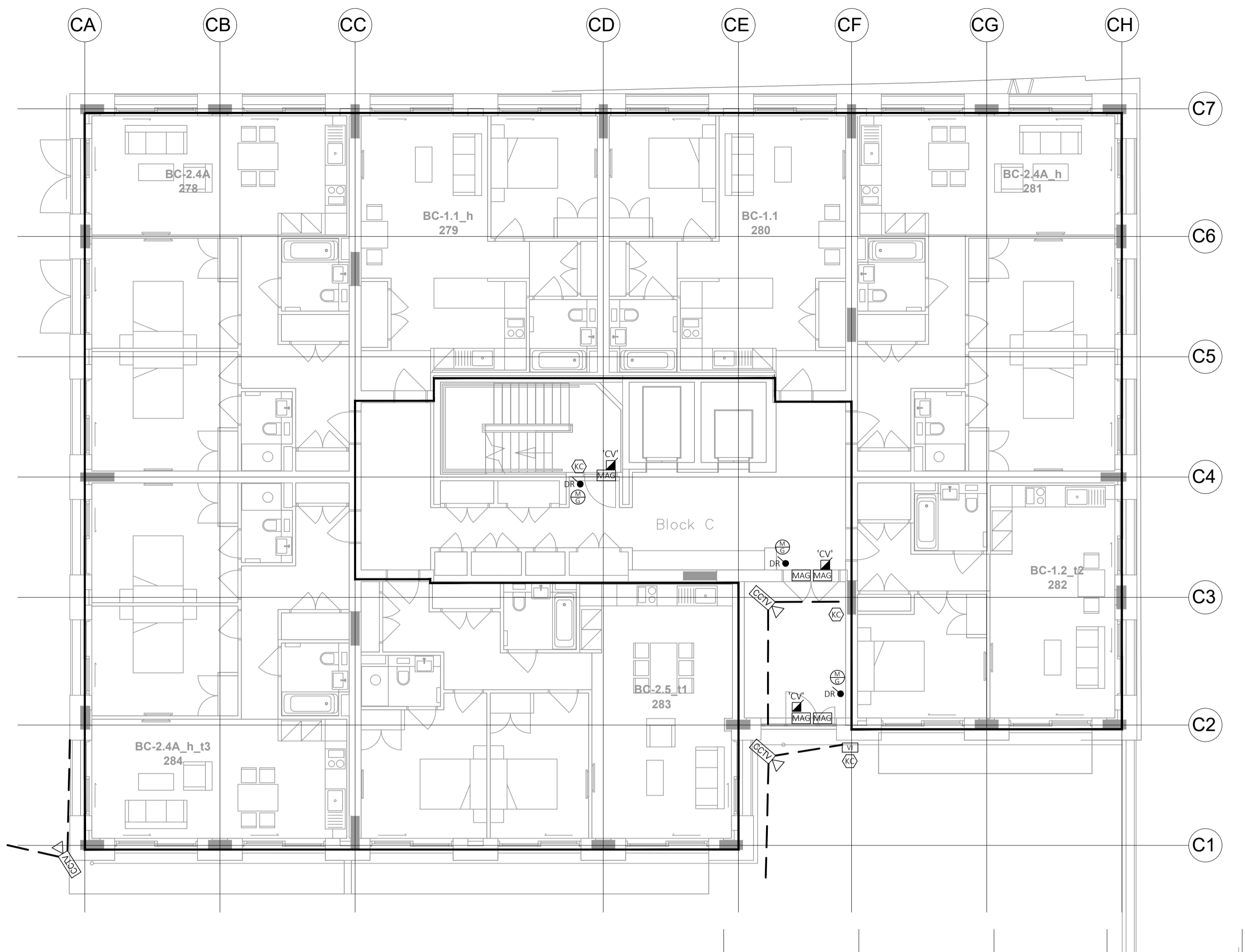
BLOCK C - LEVEL 01
