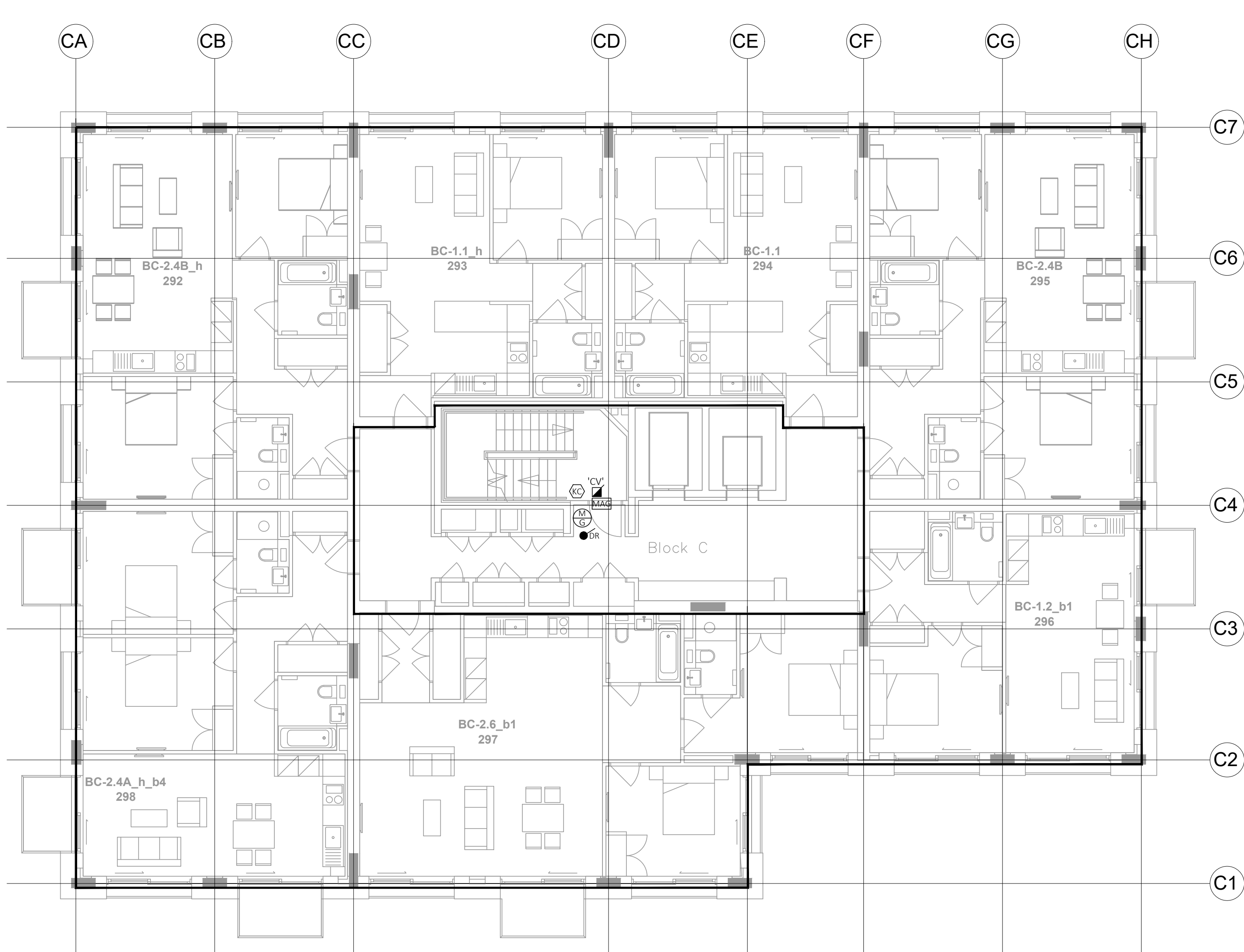
BLOCK C - LEVEL 03
