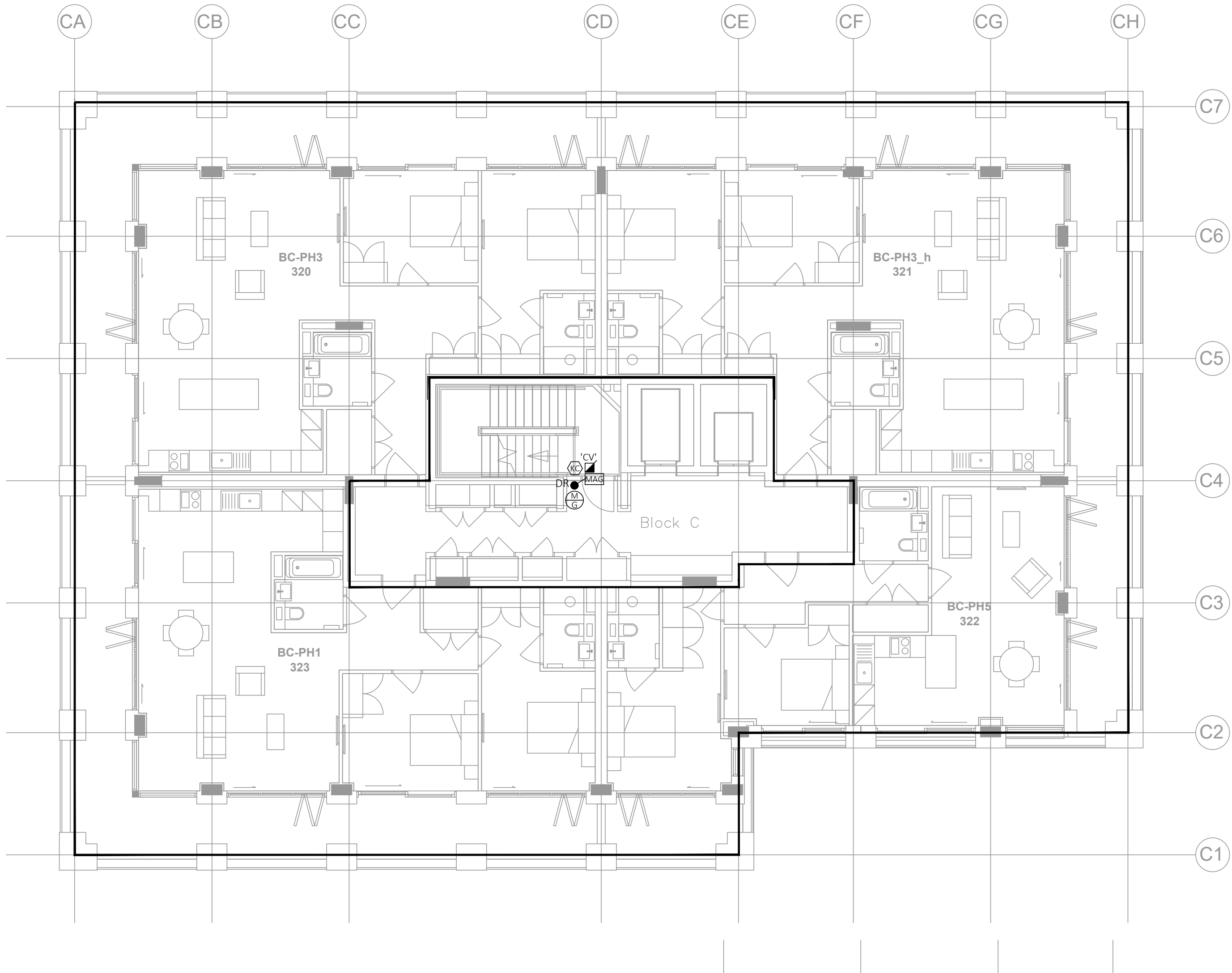
BLOCK C - LEVEL 07
