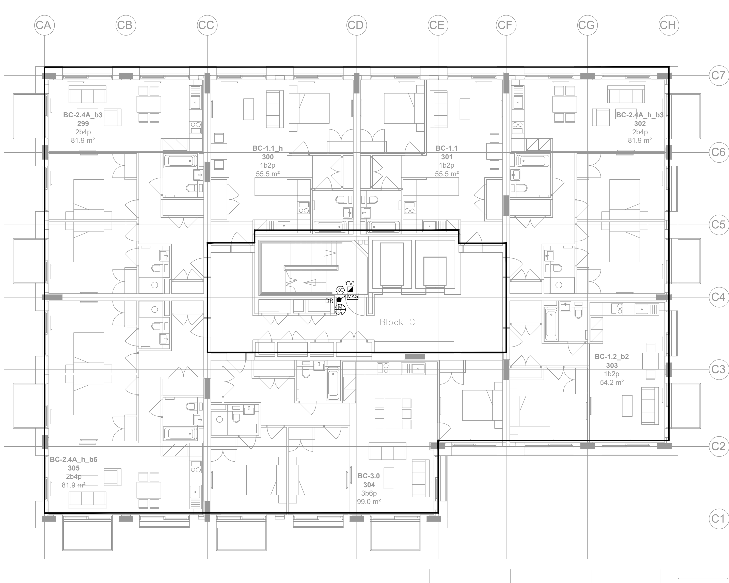
BLOCK C - LEVEL 04
