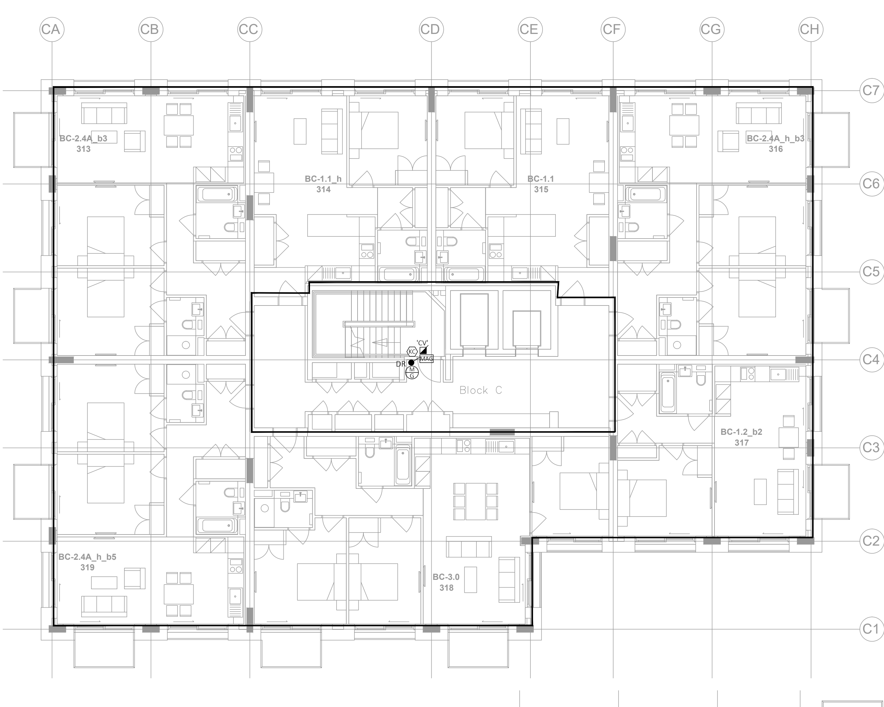
BLOCK C - LEVEL 06
