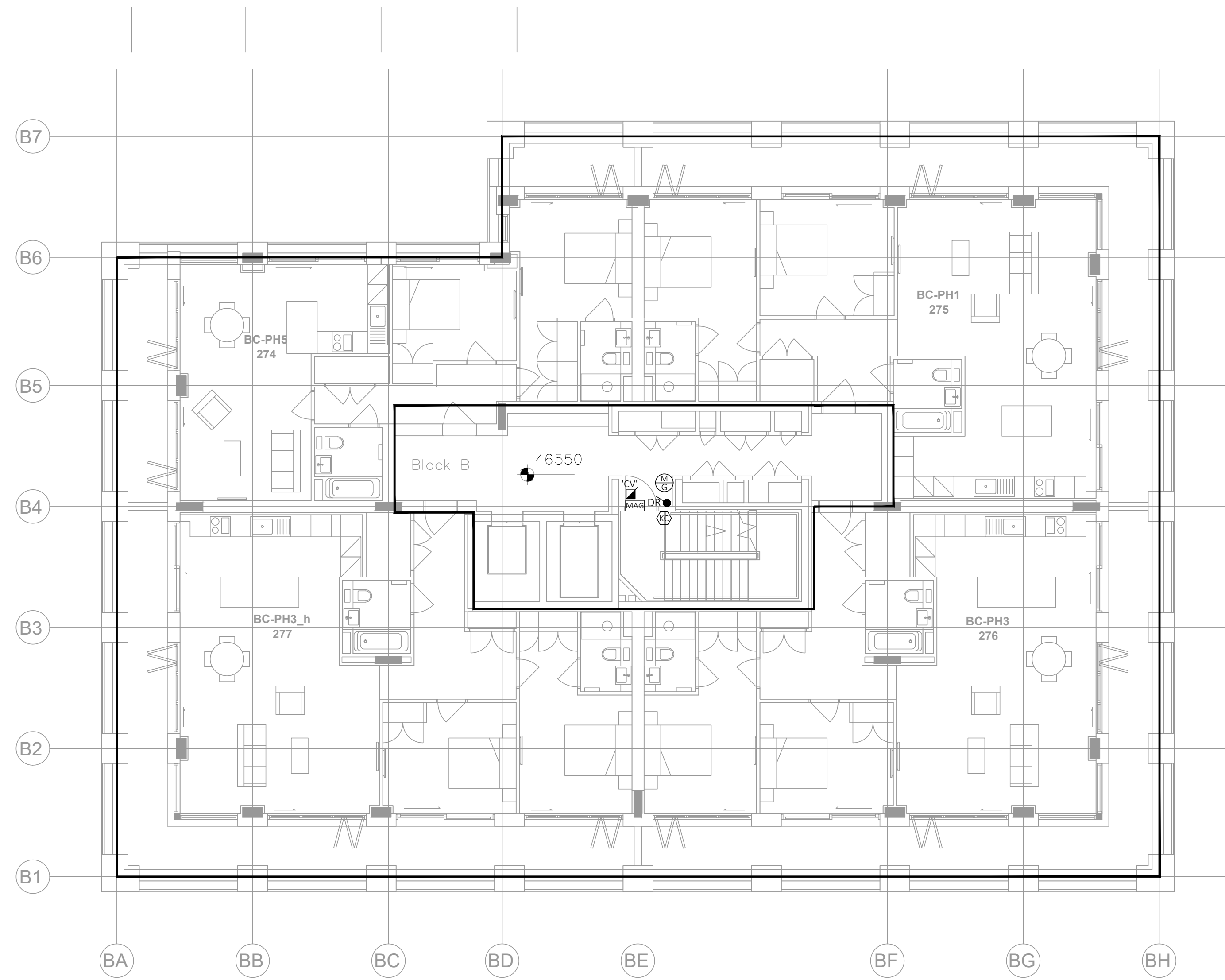
BLOCK B - LEVEL 09
