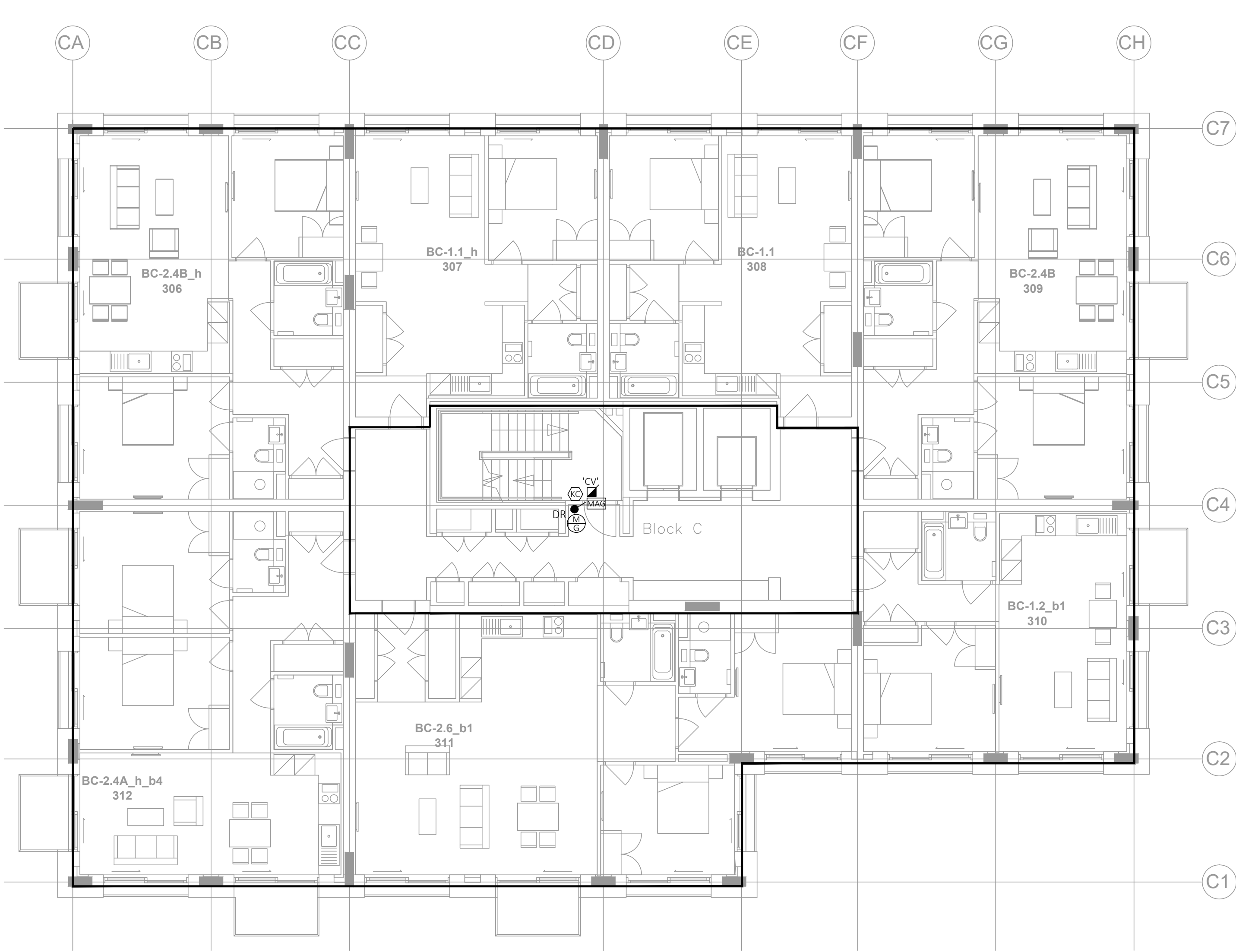
BLOCK C - LEVEL 05
