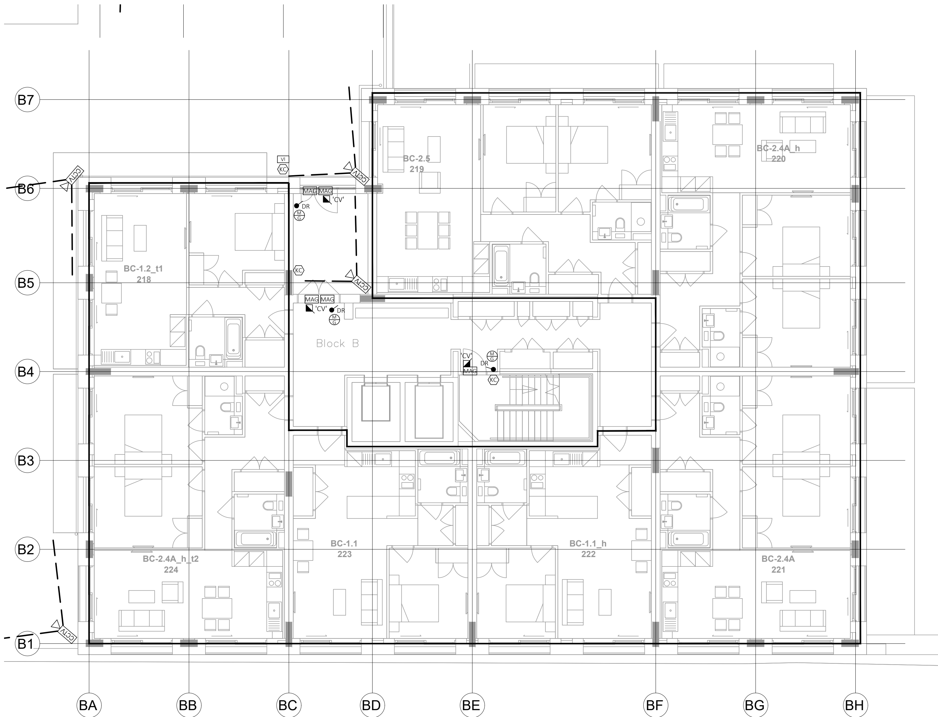
BLOCK B - LEVEL 01
