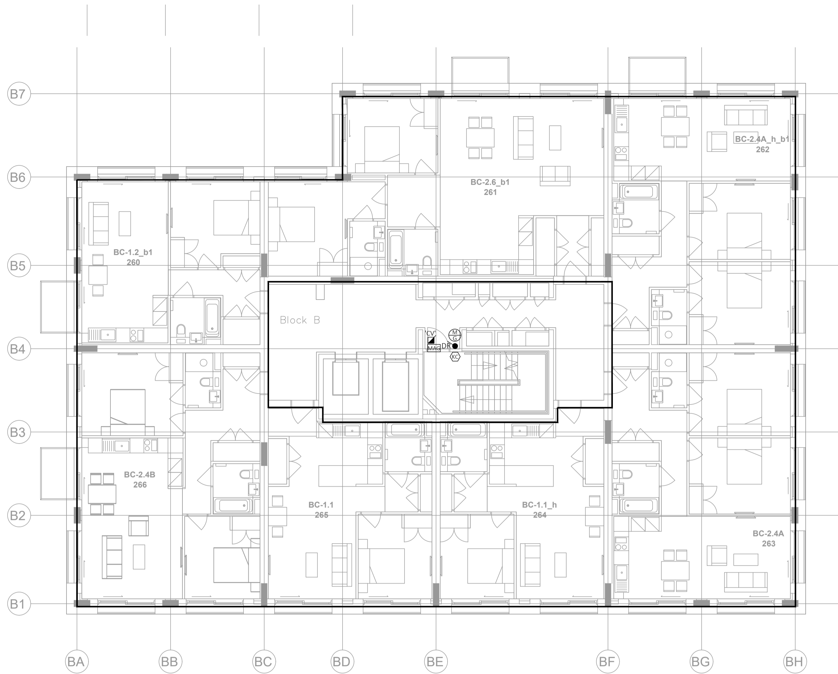
BLOCK B - LEVEL 07
