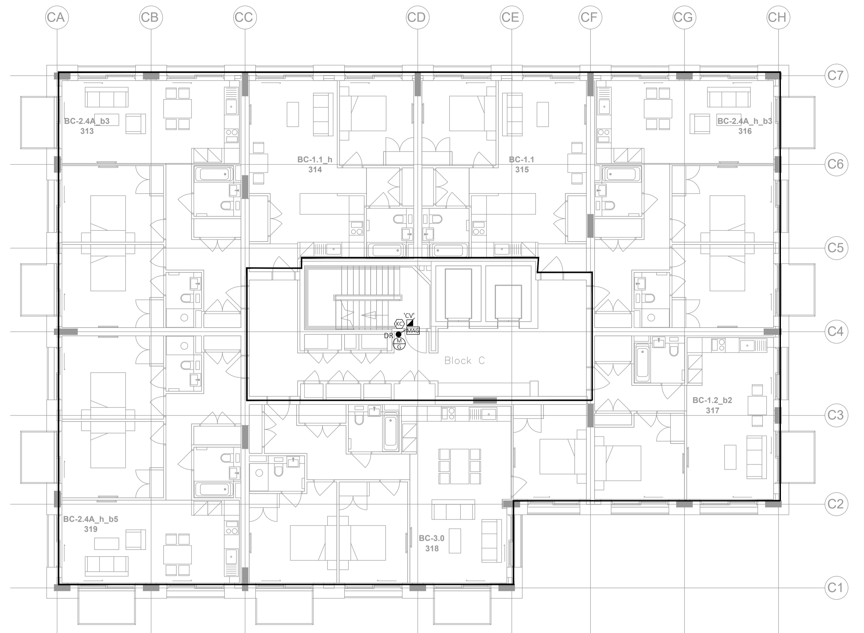
BLOCK C - LEVEL 06
