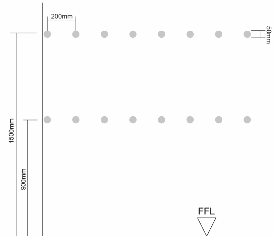
Manifestation Layout
