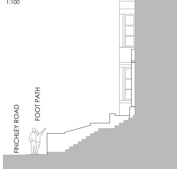
4 SECTION -B EXISTING 1:100
