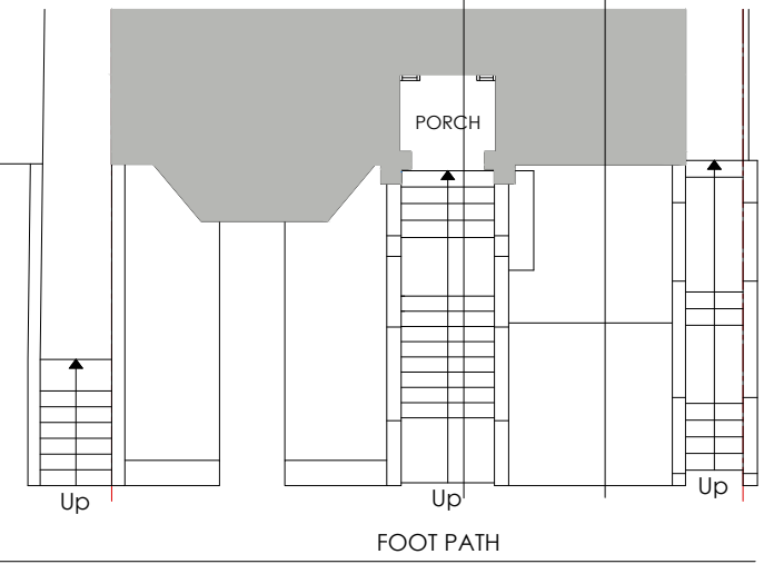
3 UPPER GROUND FLOOR PLAN EXISTING 1:100
