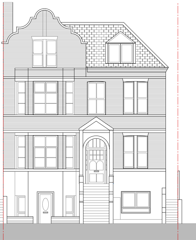
1 FRONT ELEVATION EXISTING 1:100
