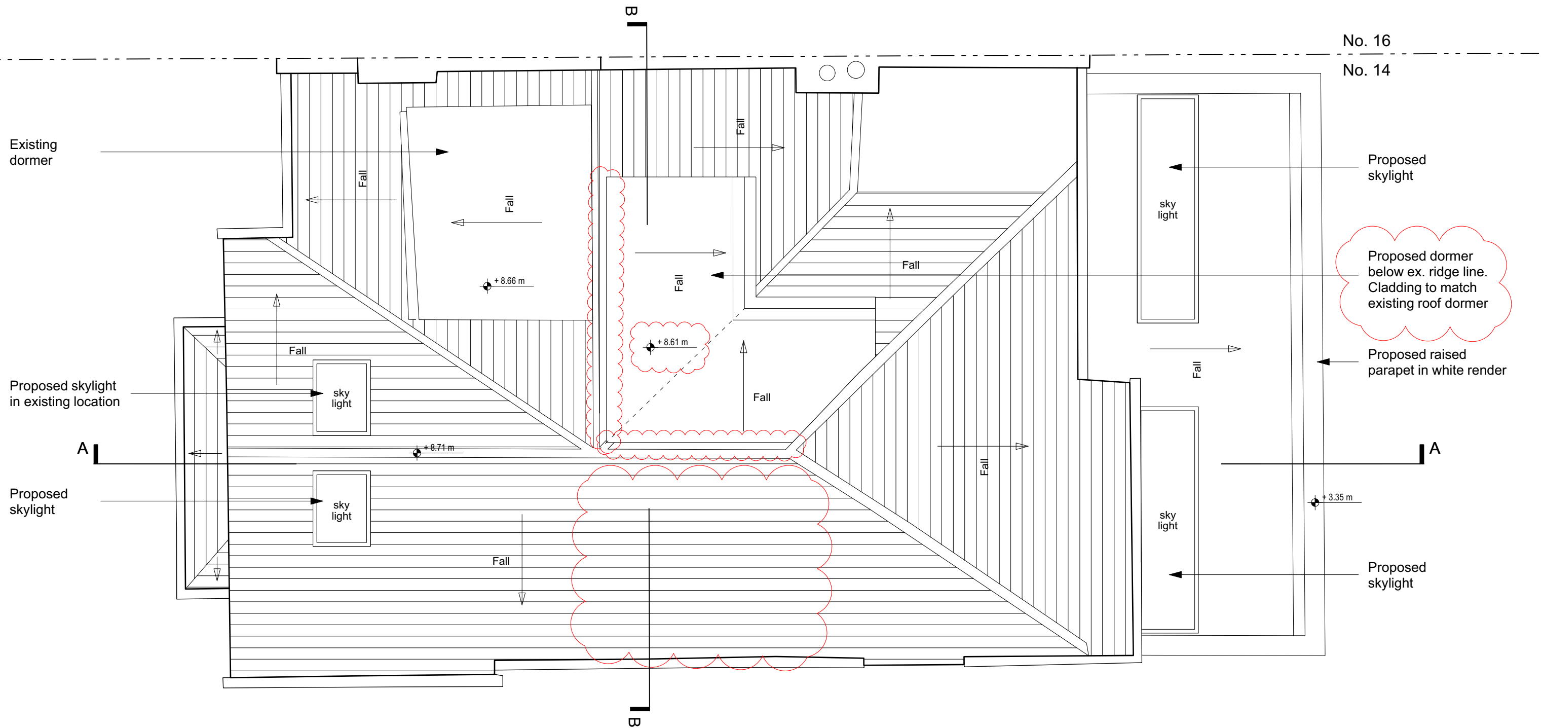
1 PROPOSED ROOF PLAN Scale: 1:50
