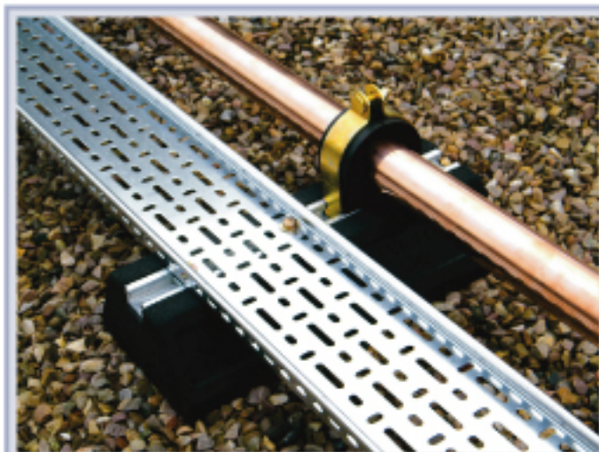
Supporting cable tray and pipework
