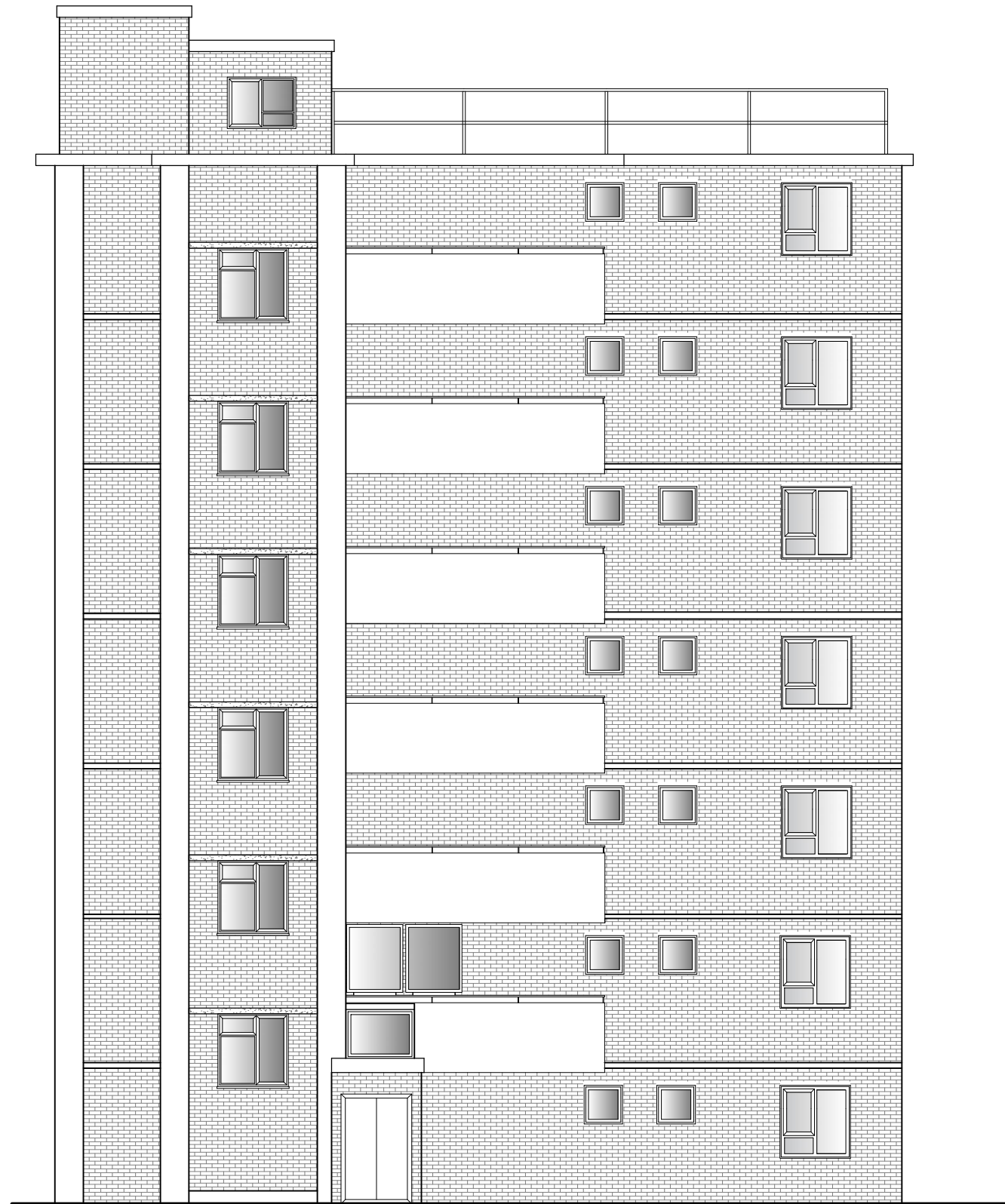
SOUTH ELEVATION
