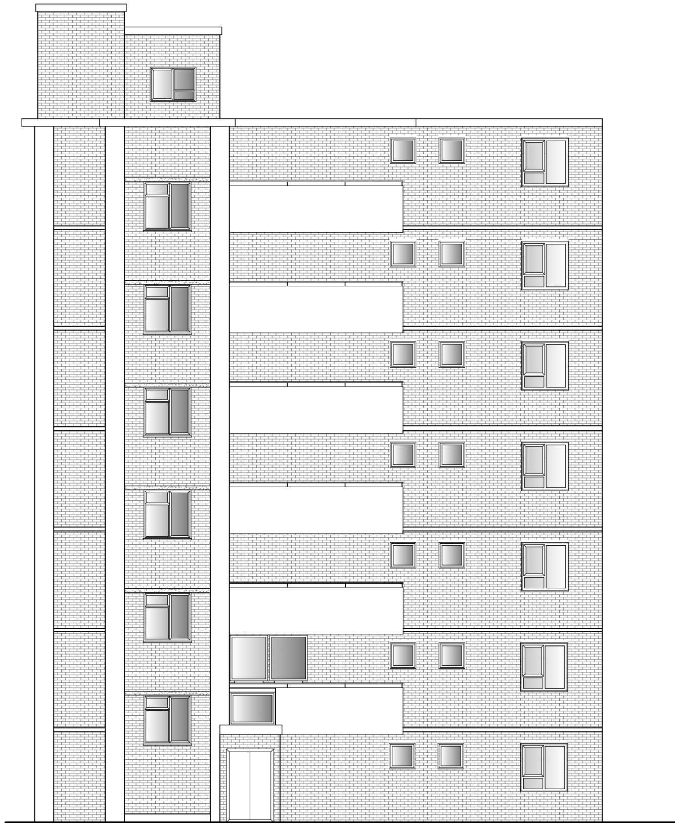
SOUTH ELEVATION
