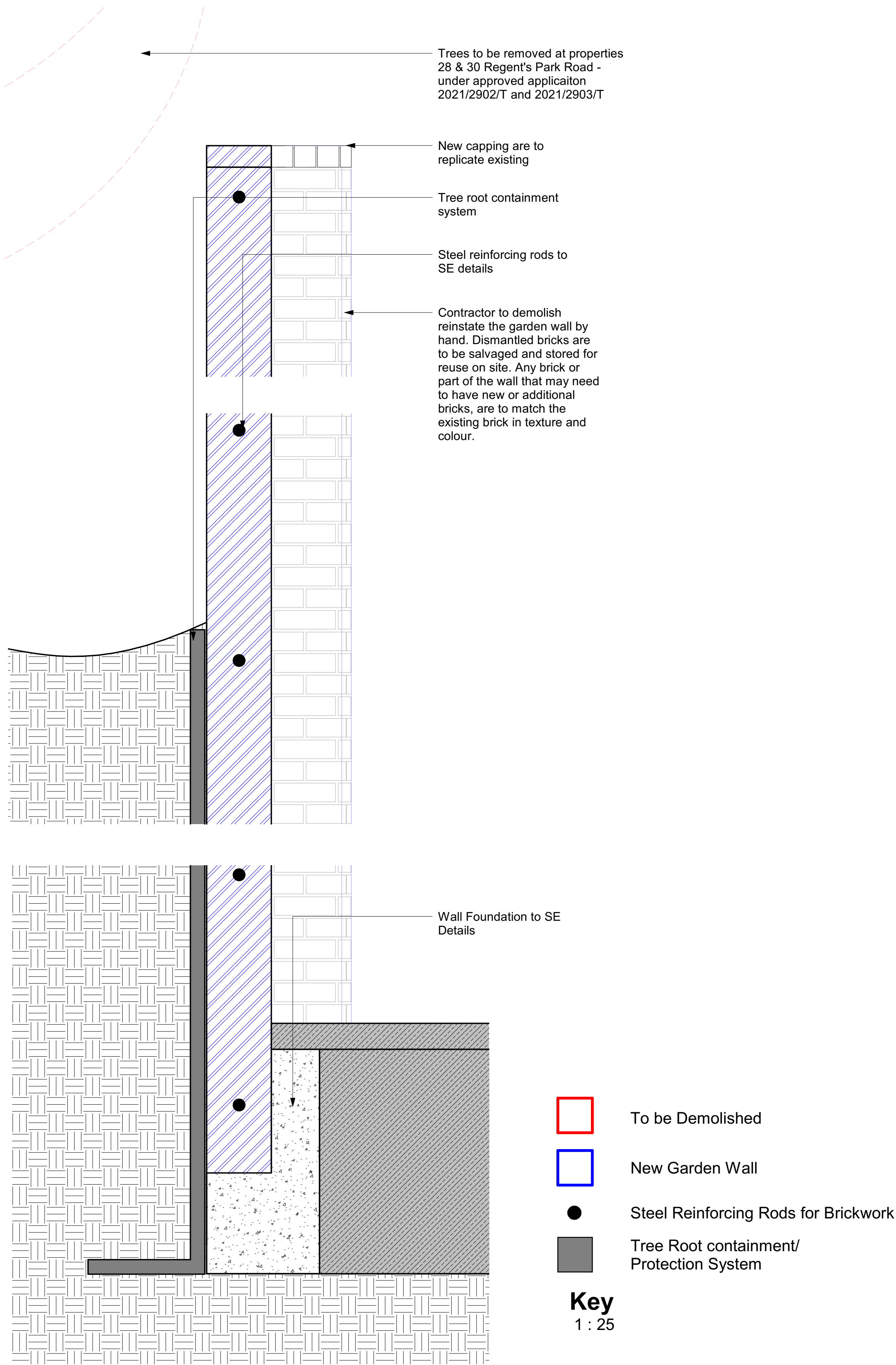
Proposed Garden Wall Section AA - Callout 1 : 10
