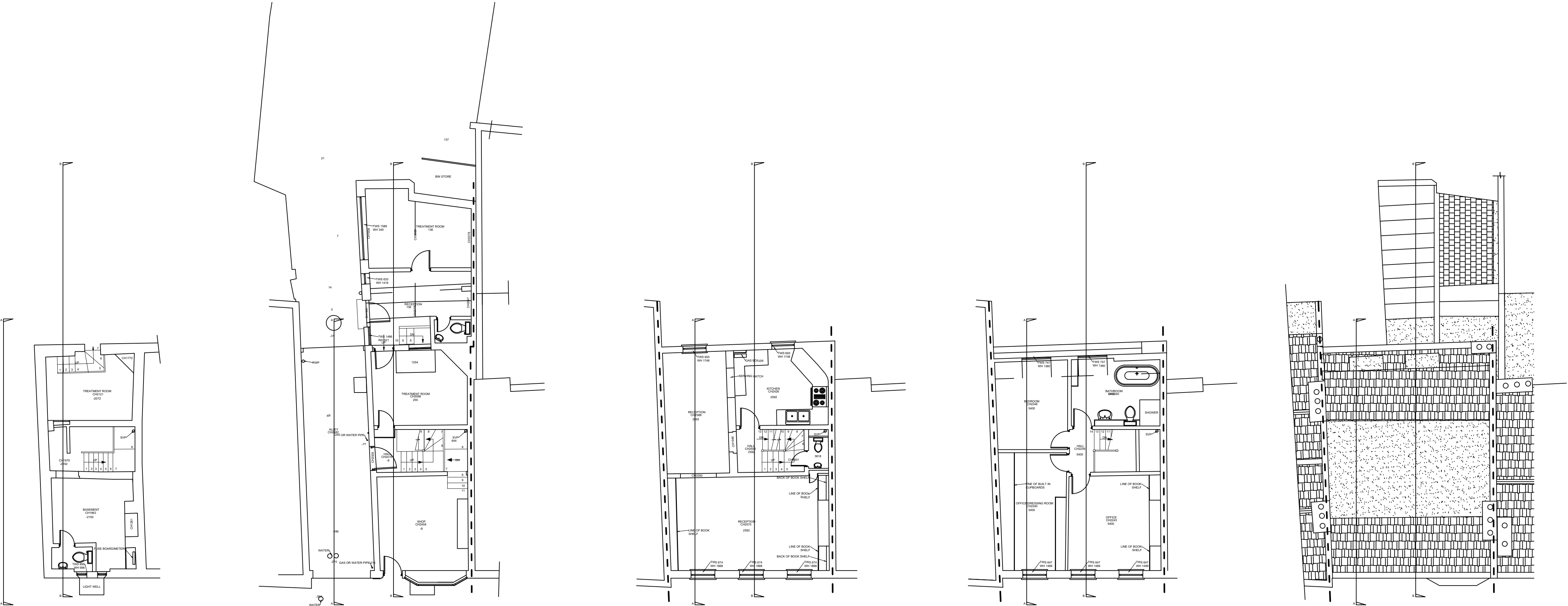
+ BASEMENT + GROUND FLOOR + FIRST FLOOR + SECOND FLOOR + ROOF PLAN
