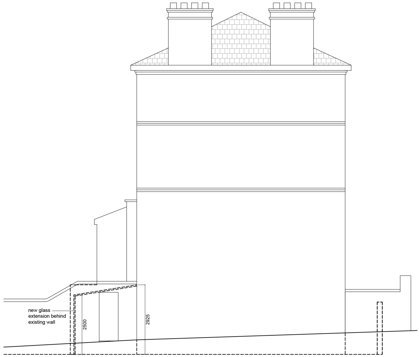
SIDE ELEVATION
