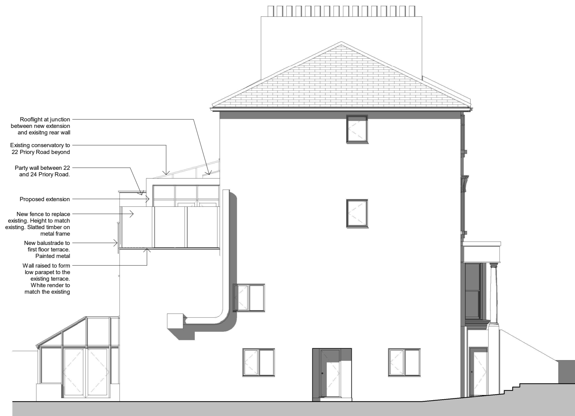
1 | Side Elevation as Proposed 1 : 100
