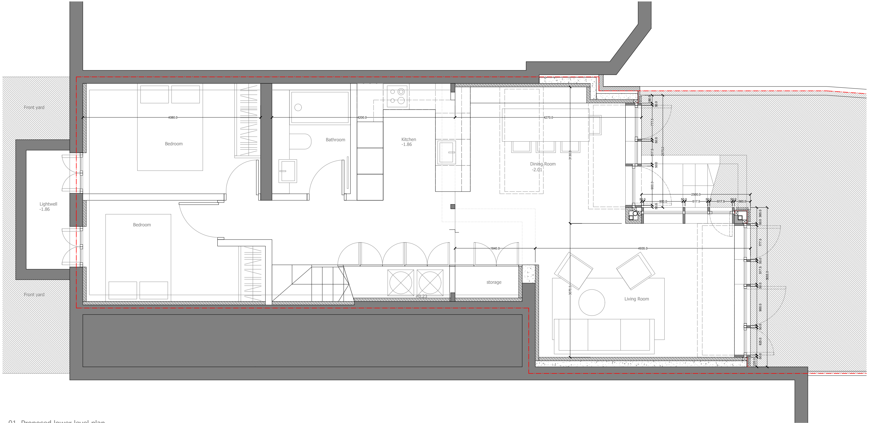
01. Proposed lower level plan
