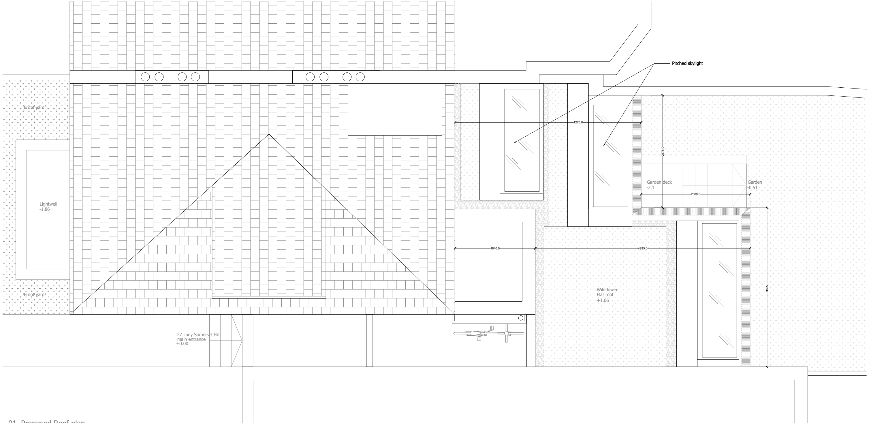
01. Proposed Roof plan
