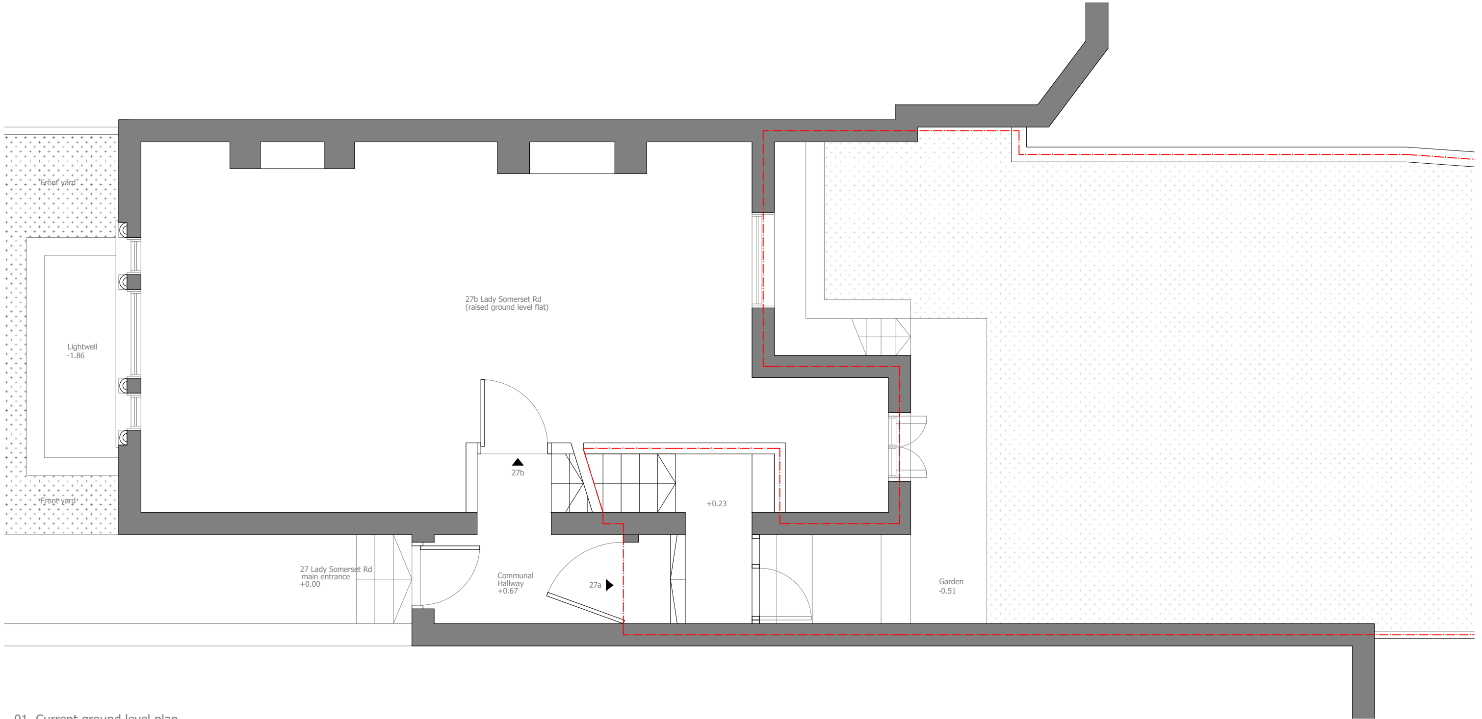
01. Current ground level plan
