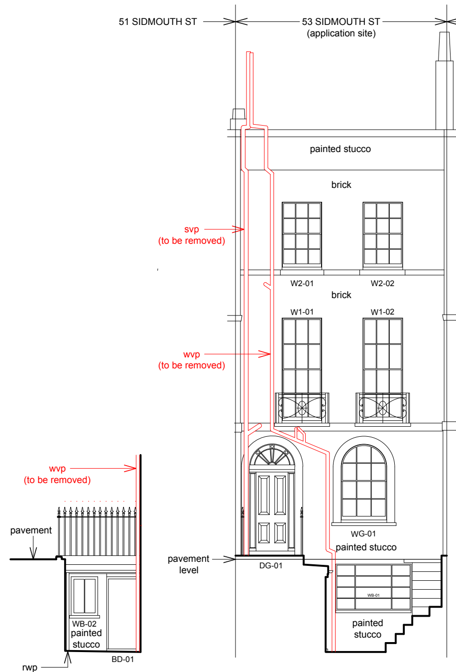
BASEMENT ENTRANCE ELEVATION to LIGHTWELL
