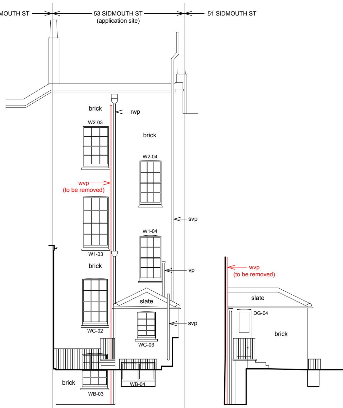
REAR ELEVATION to PRIVATE GARDEN & ST GEORGE'S GARDENS
