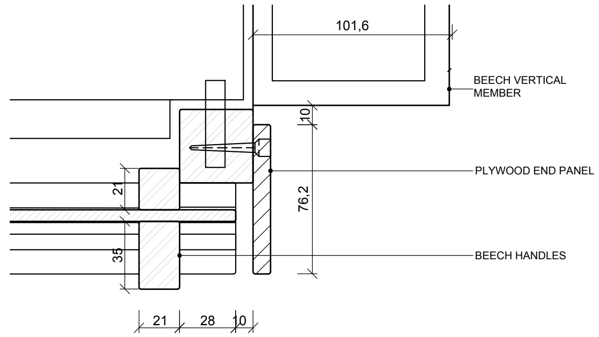
03 SCALE 1:2 PLAN DETAIL AT END PANEL OF CUPBOARD AT PART HEIGHT WALL
