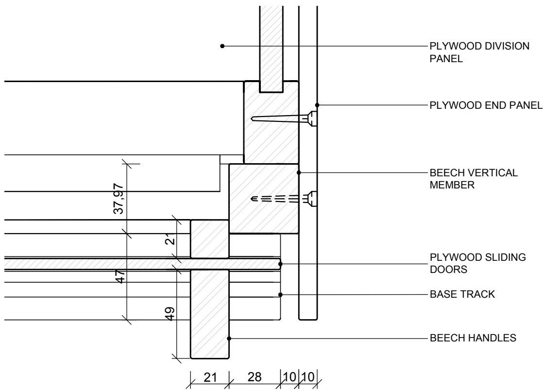
02 SCALE 1:2 PLAN DETAIL AT END PANEL OF MODIFIED CUPBOARD
