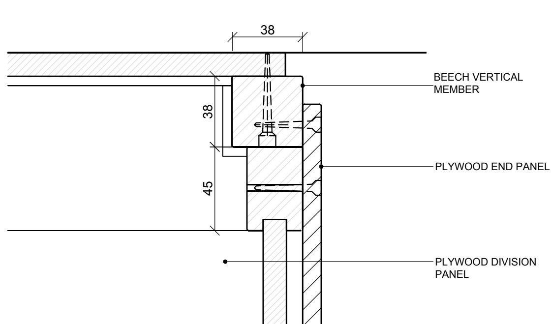
01 SCALE 1:2 PLAN DETAIL AT REAR END PANEL OF MODIFIED CUPBOARD
