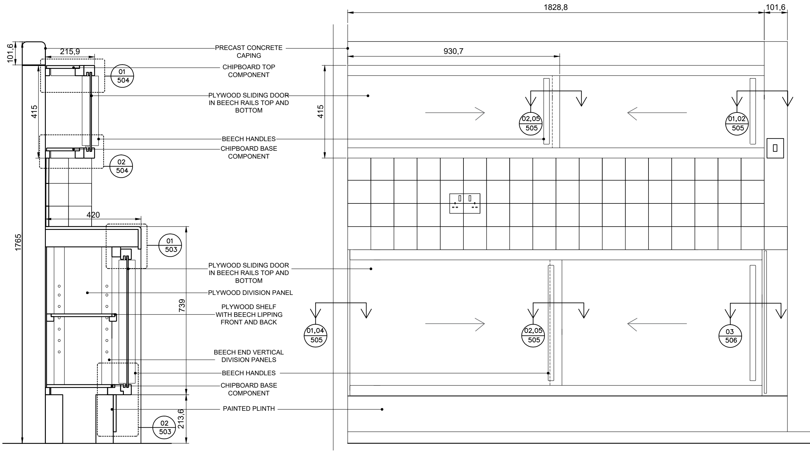
01 SCALE 1:10 CROSS SECTION
