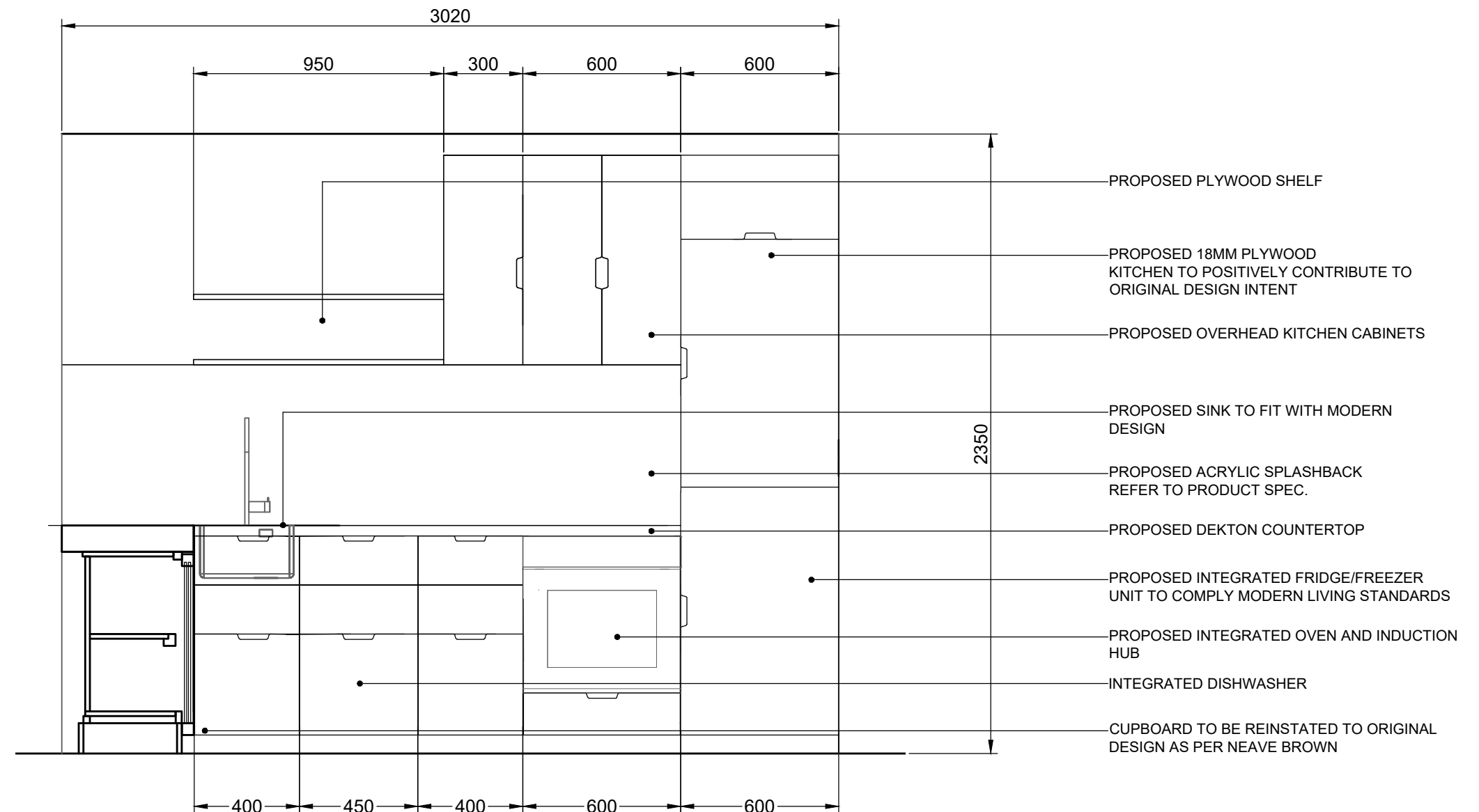
01 SCALE 1:20 PROPOSED KITCHEN ELEVATION A
