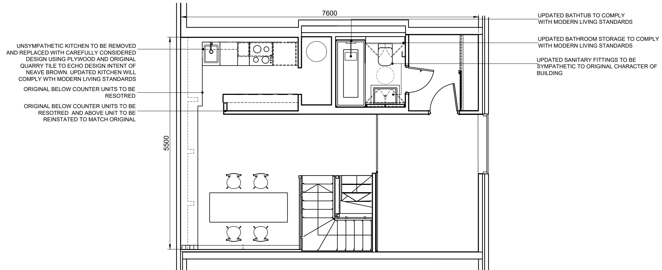
01 SCALE 1:50 PROPOSED FIRST FLOOR PLAN N 0 0.5m 1m 2m 1:50
